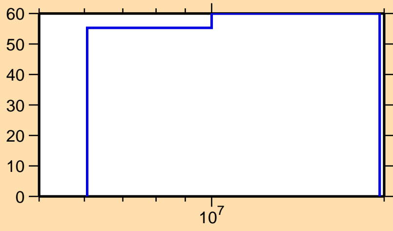
\Delta\sigma/\sigma vs. E for ^{41}\text{Cl}(n,\gamma)
