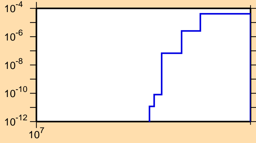
\sigma vs. E for ^{42}\text{Cl}(n,n\alpha)
