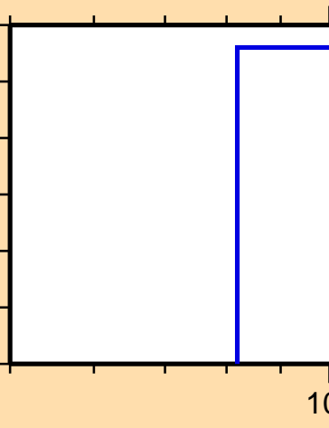
\sigma vs. E for ^{42}\text{Cl}(n,2n\alpha)
