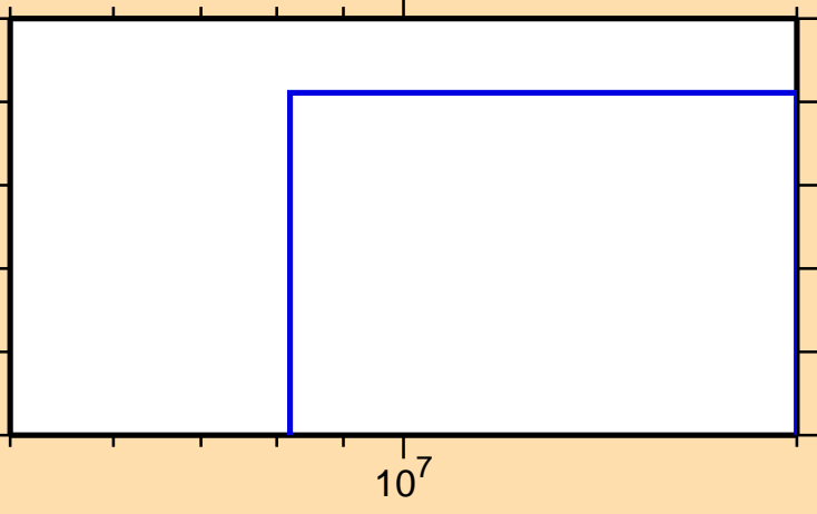
\sigma vs. E for ^{42}\text{Cl}(n,nt)
