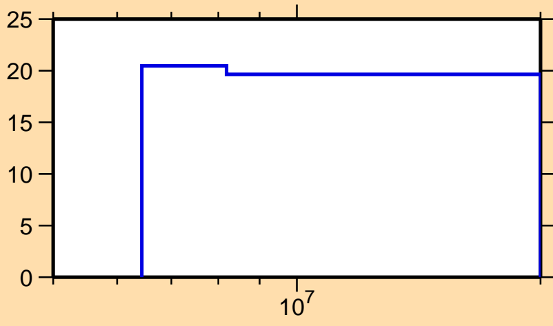
\Delta\sigma/\sigma vs. E for ^{42}\text{Cl}(n,el.)
