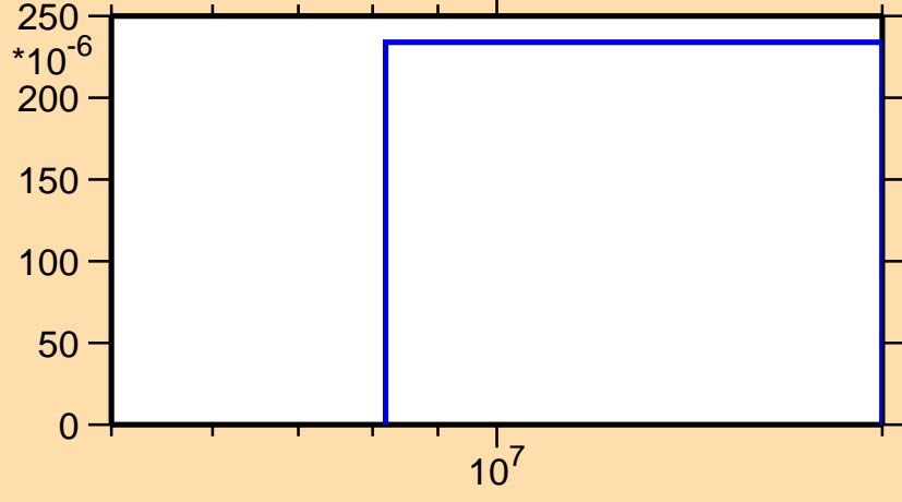
\sigma vs. E for ^{42}\text{Cl}(n,t)
