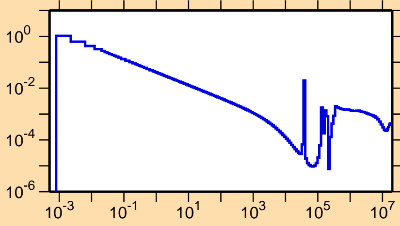
\sigma vs. E for ^{43}\text{Cl}(n,\gamma)
