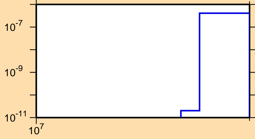
\sigma vs. E for ^{43}\text{Cl}(n,nt)
