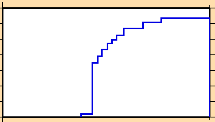
\sigma vs. E for ^{43}\text{Cl}(n,3n)
