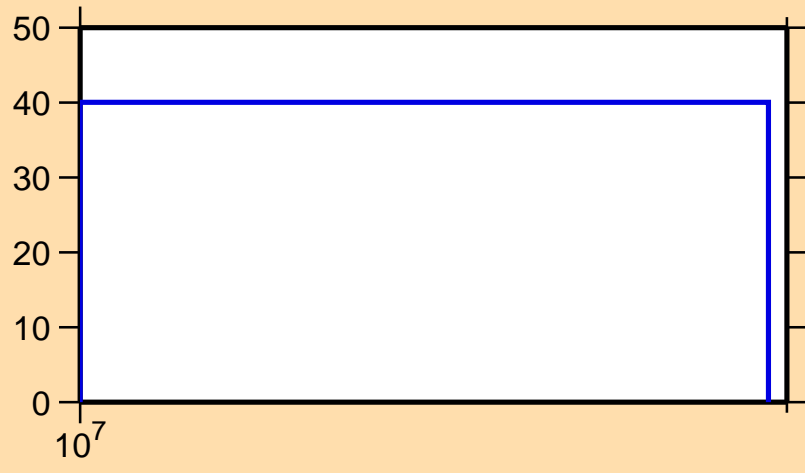
\Delta\sigma/\sigma vs. E for ^{43}\text{Cl}(n,n_1)
