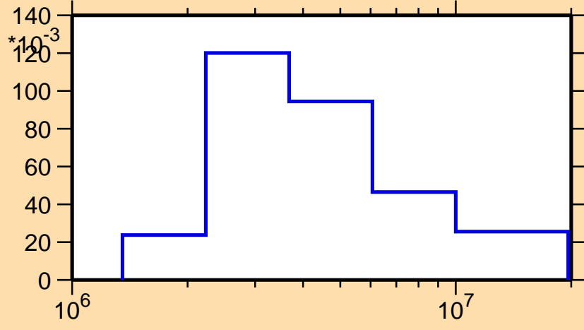
\sigma vs. E for ^{43}\text{Cl}(n,n_4)
