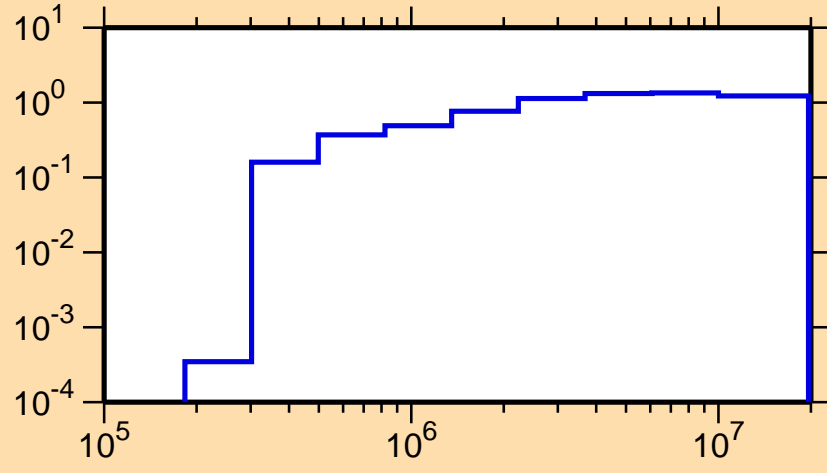
\sigma vs. E for ^{43}\text{Cl}(n,\text{nonel.})
