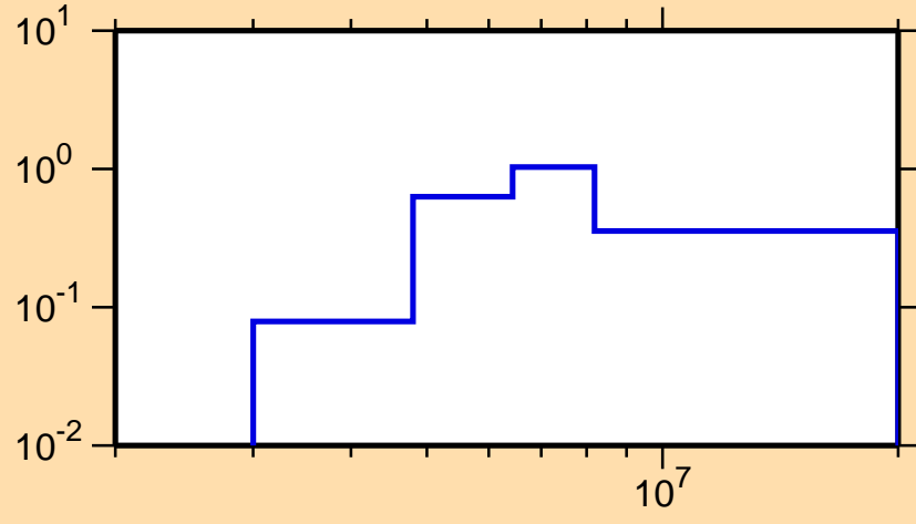
\sigma vs. E for ^{43}\text{Cl}(n,n\text{cont.})
