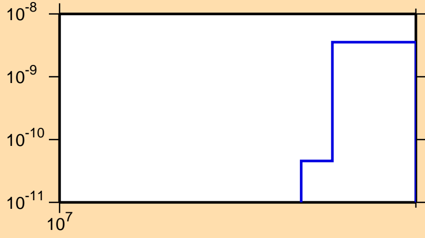
\sigma vs. E for ^{232}\text{Cm}(n,3n)
