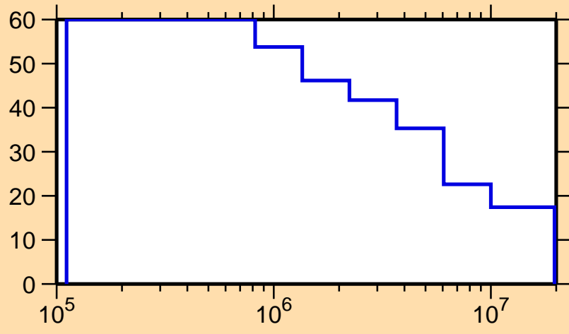
\Delta\sigma/\sigma vs. E for ^{232}\text{Cm}(n,f)
