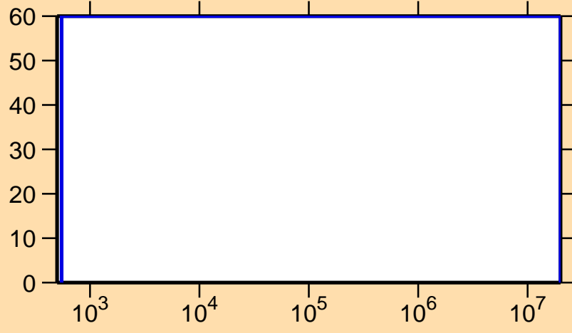
\Delta\sigma/\sigma vs. E for ^{232}\text{Cm}(n,\gamma)
