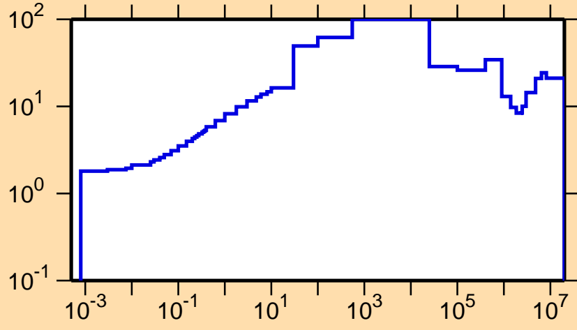
\Delta\sigma/\sigma vs. E for ^{232}\text{Cm}(n,tot.)
