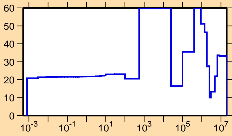
\Delta\sigma/\sigma vs. E for ^{232}\text{Cm}(n,el.)
