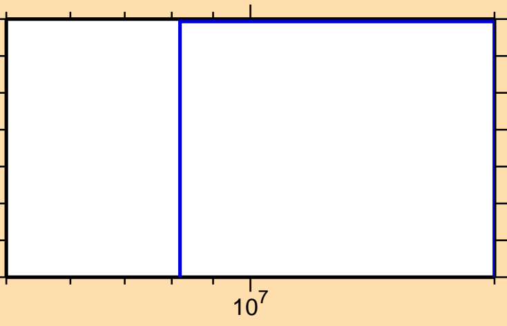
\sigma vs. E for ^{232}\text{Cm}(n,2n\alpha)
