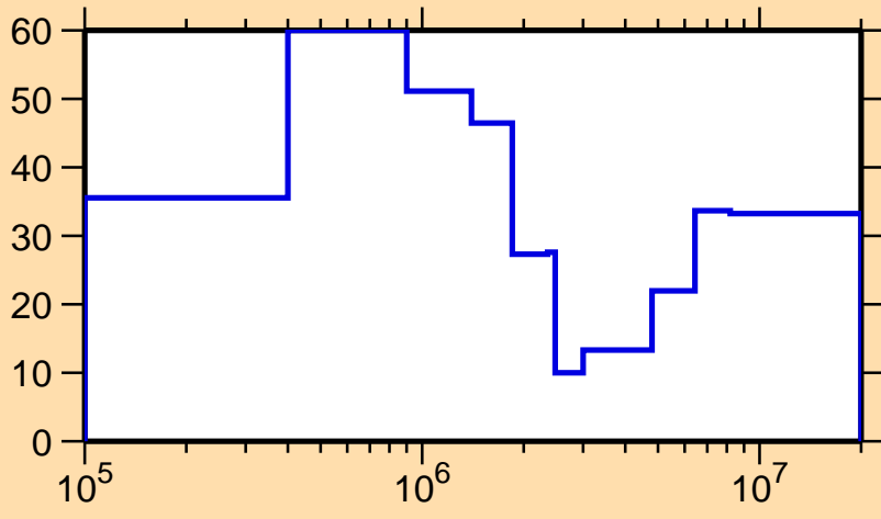
\Delta\sigma/\sigma vs. E for ^{232}\text{Cm}(n,\text{el.})
