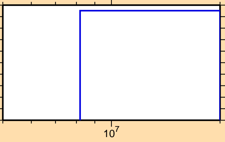
\sigma vs. E for ^{232}\text{Cm}(n,\text{He3})
