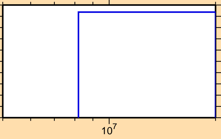
\sigma vs. E for ^{232}\text{Cm}(n,t)
