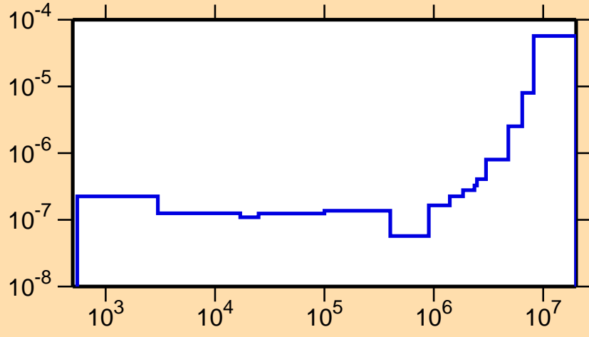
\sigma vs. E for ^{232}\text{Cm}(n,\alpha)
