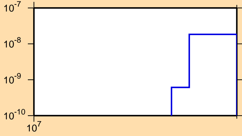
\sigma vs. E for ^{233}\text{Cm}(n,3n\alpha)
