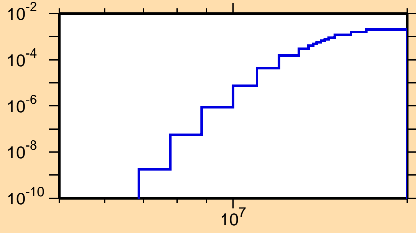
\sigma vs. E for ^{233}\text{Cm}(\text{mt117})
