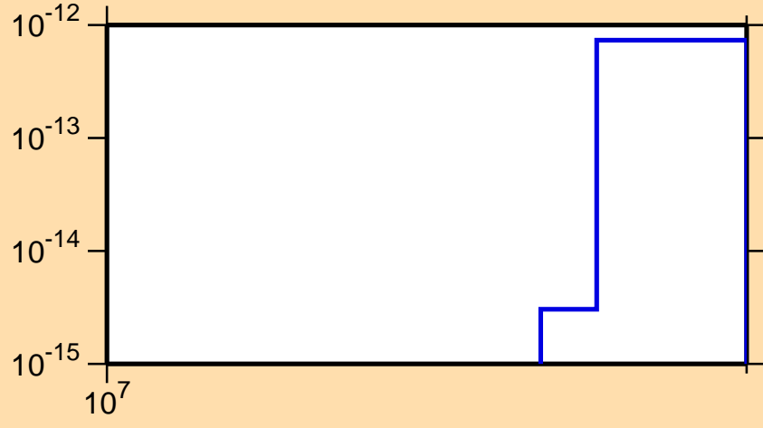
\sigma vs. E for ^{233}\text{Cm}(n,nt)
