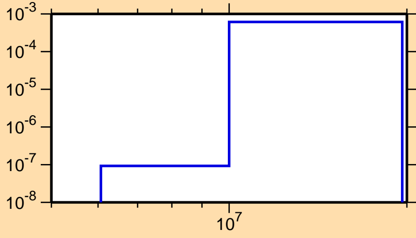
\sigma vs. E for ^{233}\text{Cm}(\text{mt117})
