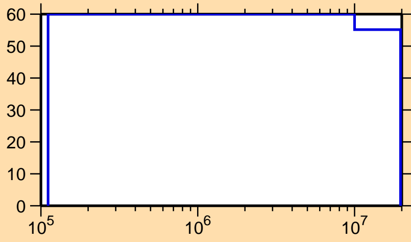
\Delta\sigma/\sigma vs. E for ^{233}\text{Cm}(n,ncont.)
