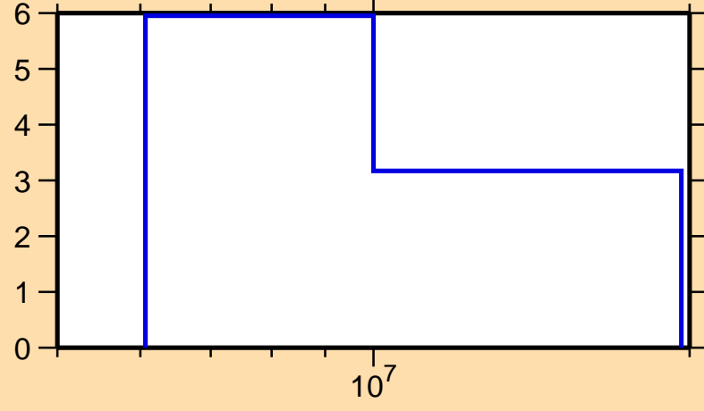
\Delta\sigma/\sigma vs. E for ^{233}\text{Cm}(n,\text{nonel.})
