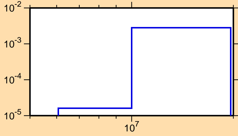
\sigma vs. E for ^{233}\text{Cm}(n,2n\alpha)
