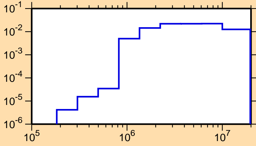
\sigma vs. E for ^{233}\text{Cm}(n,n\text{cont.})
