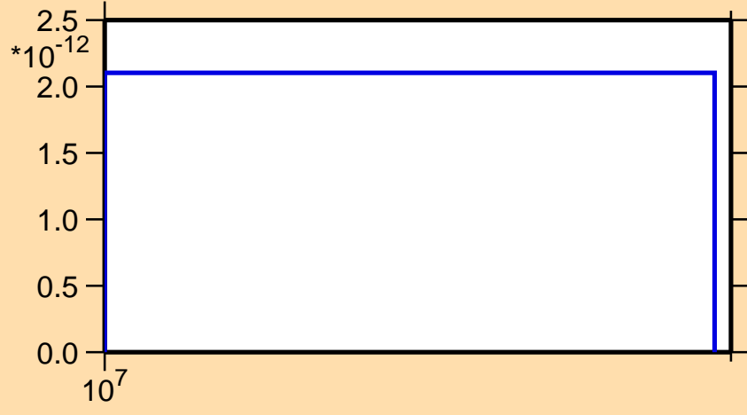
\sigma vs. E for ^{233}\text{Cm}(n,nd)
