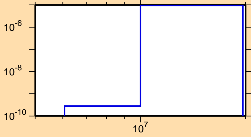
\sigma vs. E for ^{234}\text{Cm}(\text{mt117})
