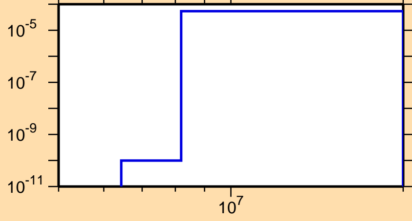
\sigma vs. E for ^{234}\text{Cm}(n,d)
