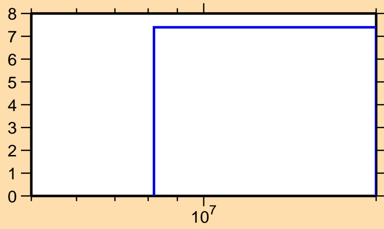
\Delta\sigma/\sigma vs. E for ^{234}\text{Cm}(n,\text{tot.})
