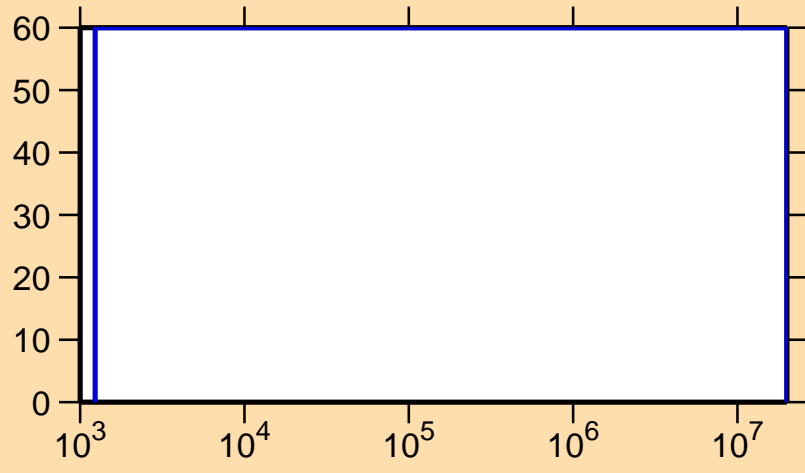
\Delta\sigma/\sigma vs. E for ^{235}\text{Cm}(n,p)
