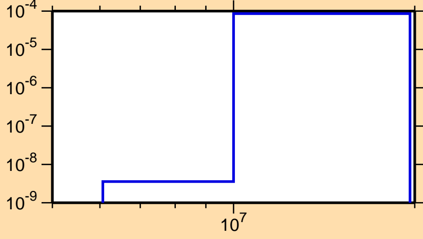
\sigma vs. E for ^{235}\text{Cm}(\text{mt117})
