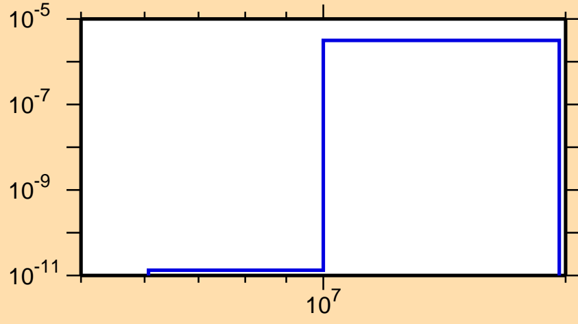
\sigma vs. E for ^{235}\text{Cm} (mt 45)
