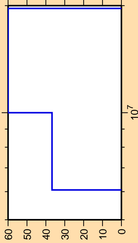
\Delta\sigma/\sigma vs. E for ^{235}\text{Cm} (mt 45)
