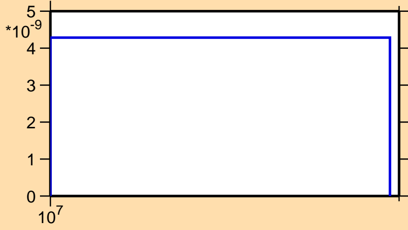
\sigma vs. E for ^{235}\text{Cm}(n,3n\alpha)
