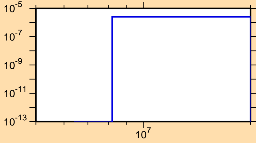
\sigma vs. E for ^{235}\text{Cm}(\text{mt 45})
