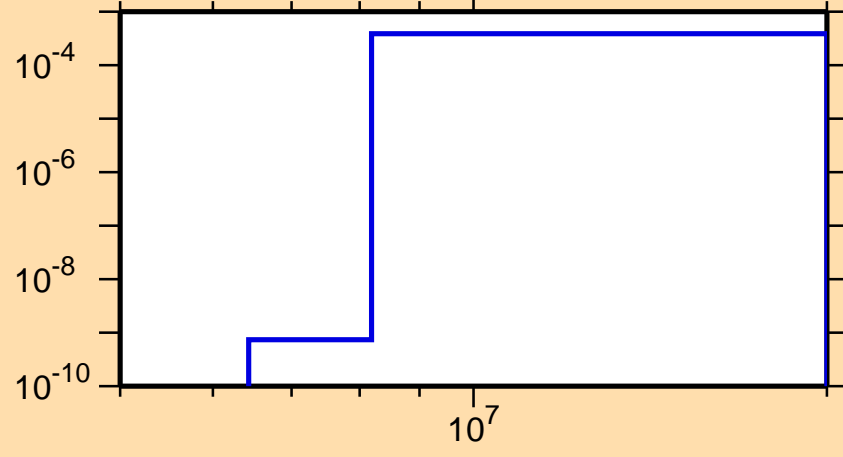
\sigma vs. E for ^{235}\text{Cm}(n,d)
