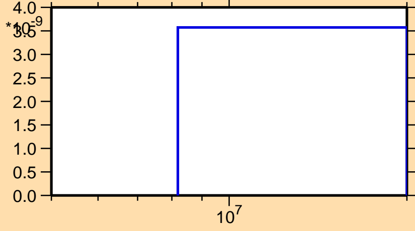
\sigma vs. E for ^{235}\text{Cm}(n,3n\alpha)
