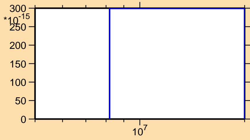
\sigma vs. E for ^{235}\text{Cm}(n,nt)
