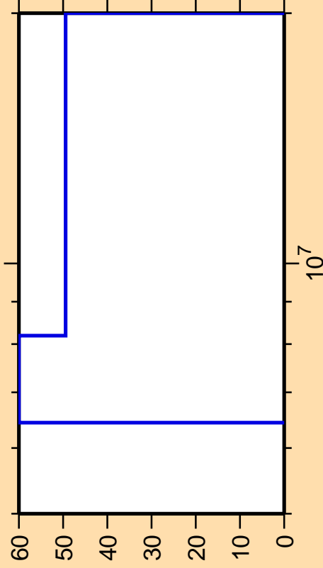
\Delta\sigma/\sigma vs. E for ^{235}\text{Cm}(\text{mt117})
