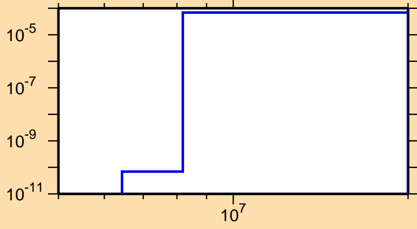
\sigma vs. E for ^{235}\text{Cm}(\text{mt117})
