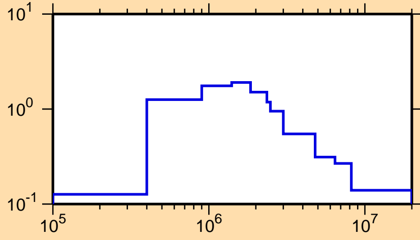
\sigma vs. E for ^{235}\text{Cm}(n,\text{inel.})
