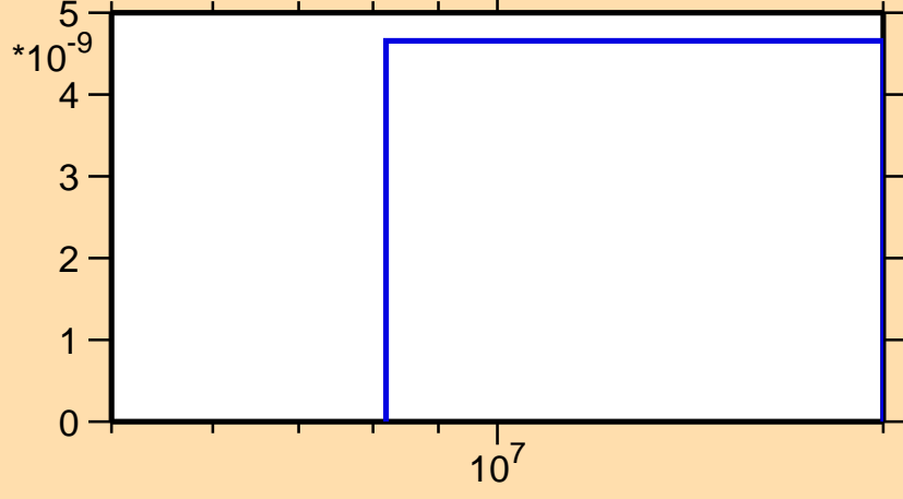
\sigma vs. E for ^{235}\text{Cm}(n,3n)
