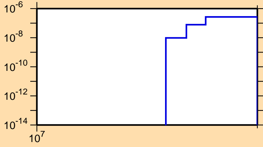
\sigma vs. E for ^{236}\text{Cm}(n,3n\alpha)
