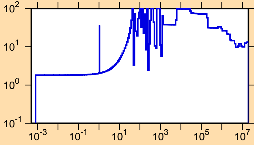
\Delta\sigma/\sigma vs. E for ^{236}\text{Cm}(n,f)
