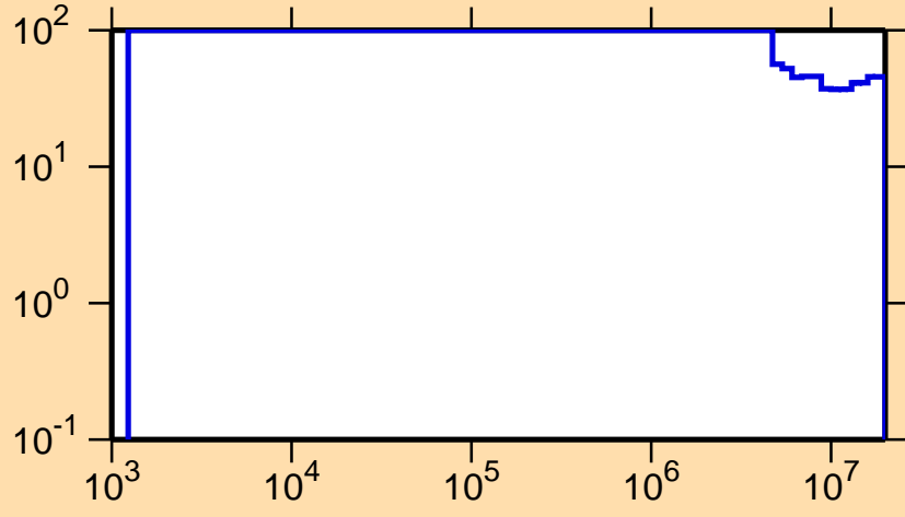
\Delta\sigma/\sigma vs. E for ^{236}\text{Cm}(n,\gamma)
