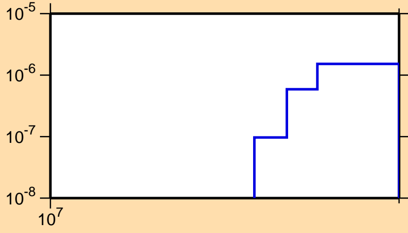
\sigma vs. E for ^{236}\text{Cm}(n,3n)
