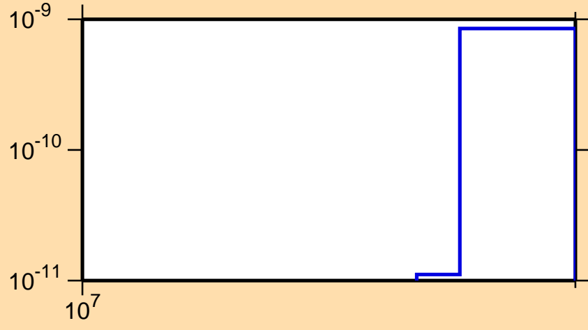
\sigma vs. E for ^{236}\text{Cm}(n,2np)
