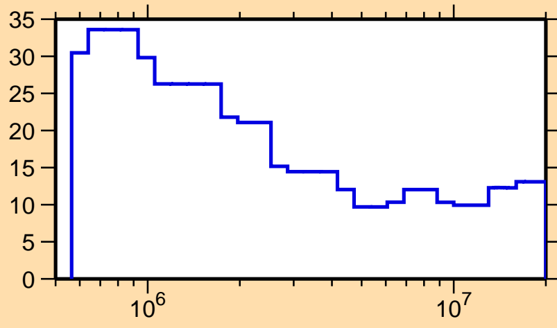
\Delta\sigma/\sigma vs. E for ^{236}\text{Cm}(n,f)
