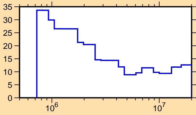
\Delta\sigma/\sigma vs. E for ^{236}\text{Cm}(n,\text{nonel.})
