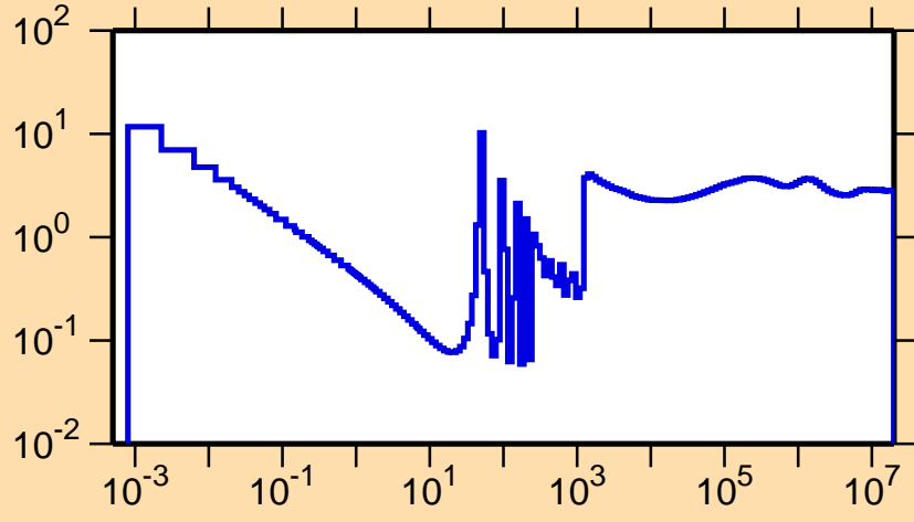
\sigma vs. E for ^{236}\text{Cm}(n,f)
