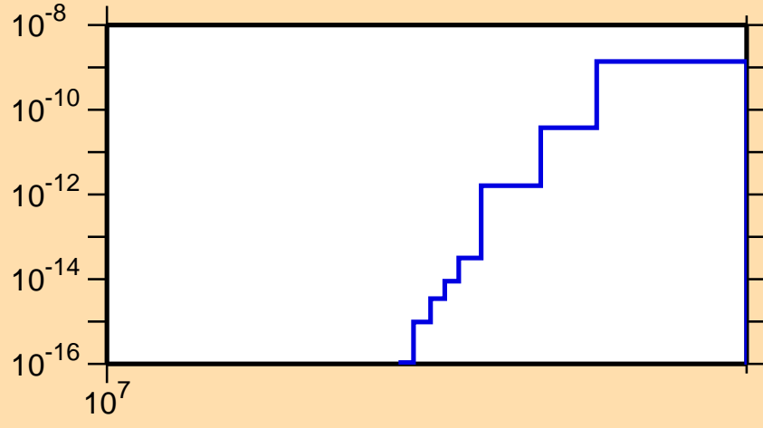
\sigma vs. E for ^{236}\text{Cm}(n,nd)
