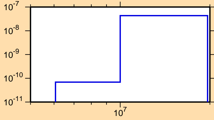
\sigma vs. E for ^{236}\text{Cm}(n,2n\alpha)
