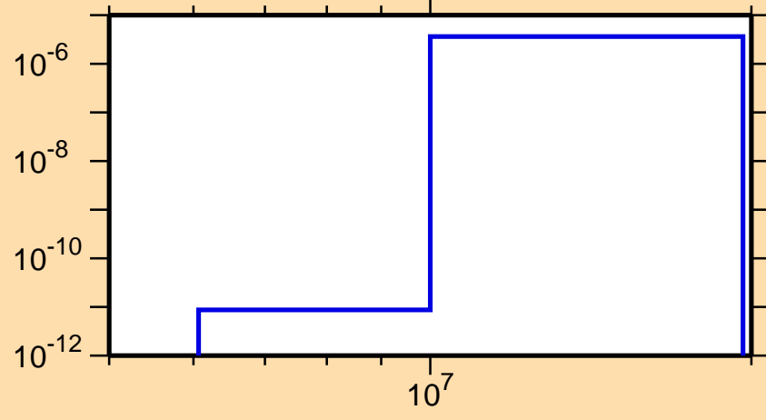
\sigma vs. E for ^{236}\text{Cm} (mt 45)
