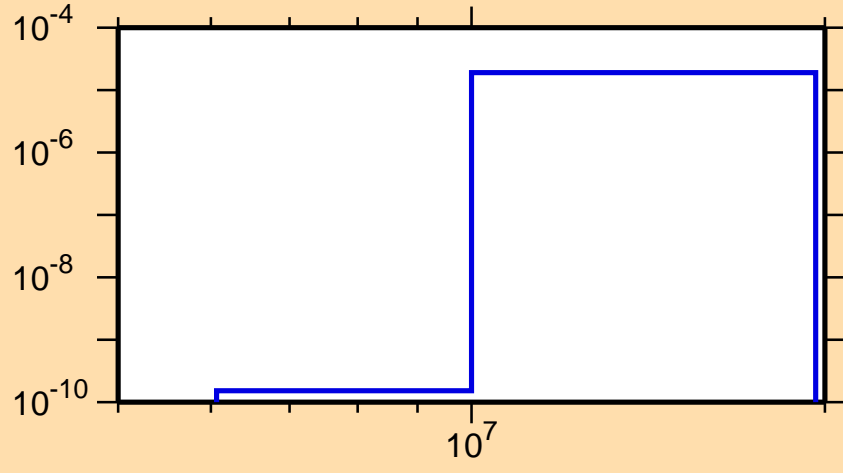
\sigma vs. E for ^{236}\text{Cm}(n,np)
