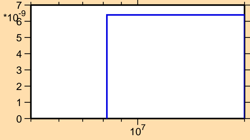
\sigma vs. E for ^{236}\text{Cm}(n,3n\alpha)
