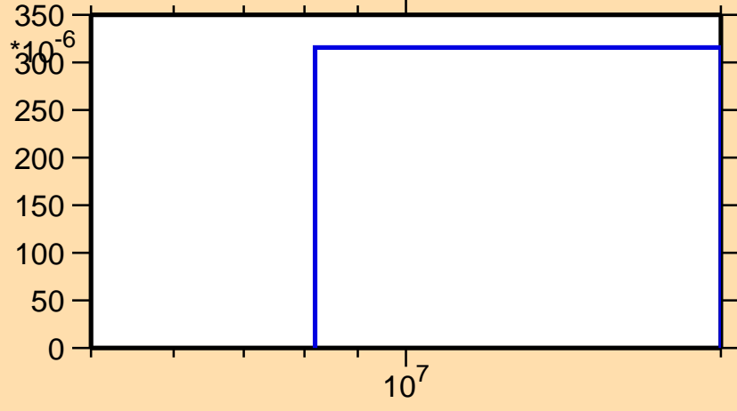
\sigma vs. E for ^{236}\text{Cm}(n,2n)
