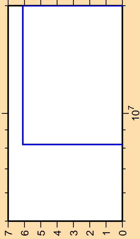
\Delta\sigma/\sigma vs. E for ^{236}\text{Cm}(n,2np)
