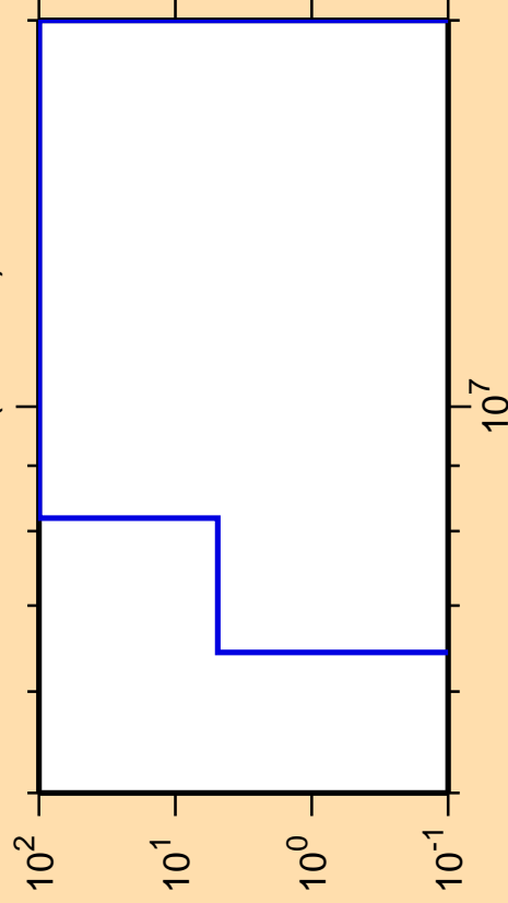
\Delta\sigma/\sigma vs. E for ^{236}\text{Cm}(\text{mt117})
