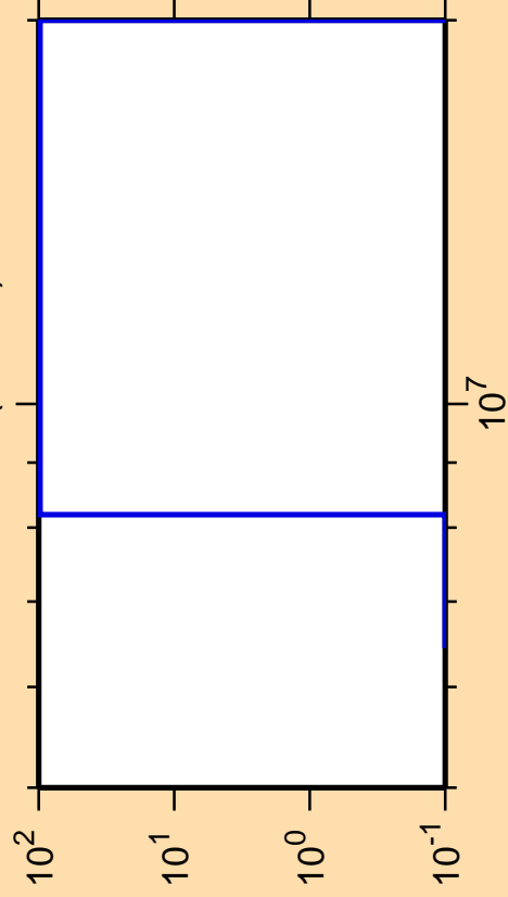
\Delta\sigma/\sigma vs. E for ^{236}\text{Cm} (mt 45)
