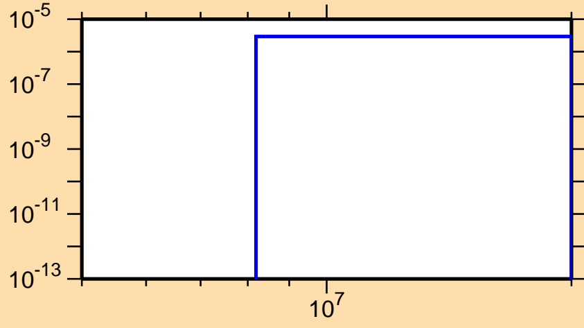
\sigma vs. E for ^{236}\text{Cm} (mt 45)
