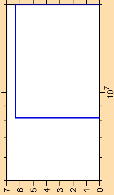
\Delta\sigma/\sigma vs. E for ^{236}\text{Cm}(n,t)
