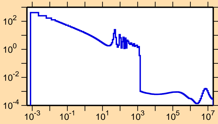
\sigma vs. E for ^{237}\text{Cm}(n,\gamma)
