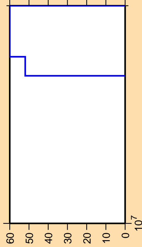
\Delta\sigma/\sigma vs. E for ^{237}\text{Cm}(n,3n\alpha)
