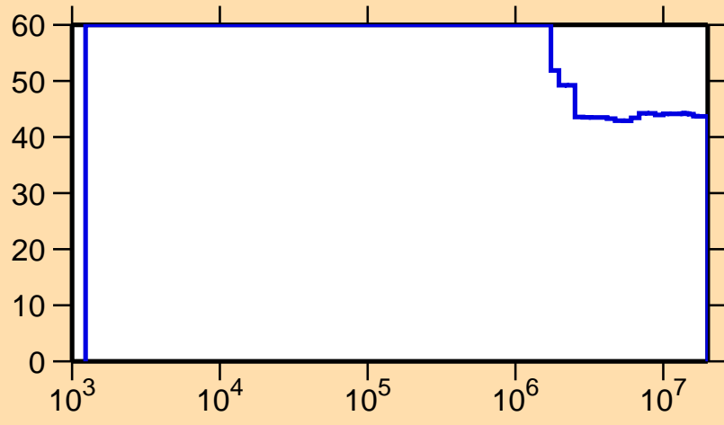
\Delta\sigma/\sigma vs. E for ^{237}\text{Cm}(n,p)
