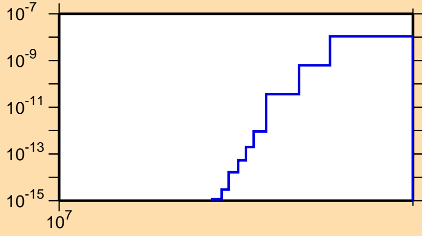
\sigma vs. E for ^{237}\text{Cm}(n,2np)
