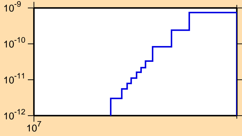
\sigma vs. E for ^{237}\text{Cm} (mt 45)
