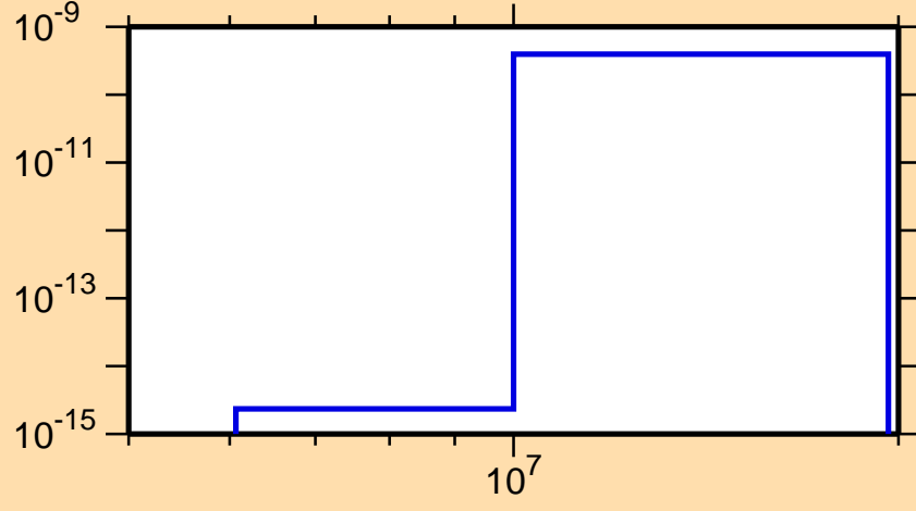
\sigma vs. E for ^{237}\text{Cm}(\text{mt117})
