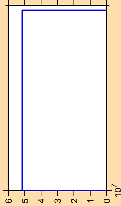
\Delta\sigma/\sigma vs. E for ^{237}\text{Cm}(n,3n\alpha)
