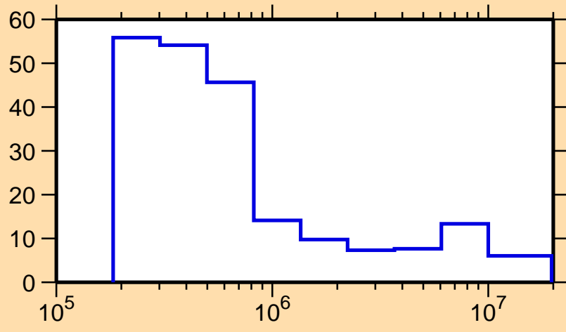
\Delta\sigma/\sigma vs. E for ^{237}\text{Cm}(n,\text{tot.})
