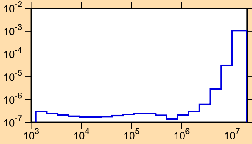
\sigma vs. E for ^{237}\text{Cm}(n,\alpha)
