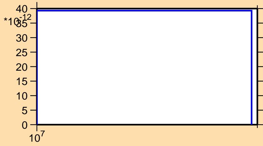
\sigma vs. E for ^{237}\text{Cm} (mt 45)
