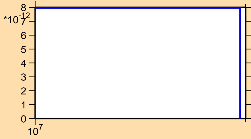
\sigma vs. E for ^{237}\text{Cm}(n,3n\alpha)
