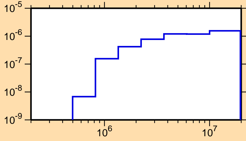
\sigma vs. E for ^{237}\text{Cm}(n,n\alpha)
