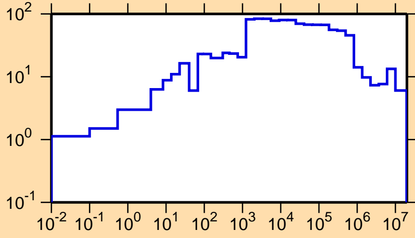
\Delta\sigma/\sigma vs. E for ^{237}\text{Cm}(n,tot.)
