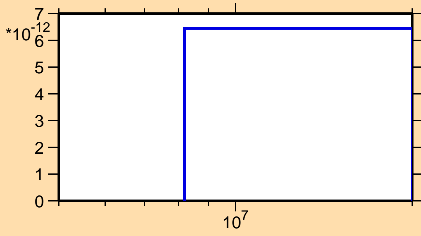
\sigma vs. E for ^{237}\text{Cm}(n,3n\alpha)
