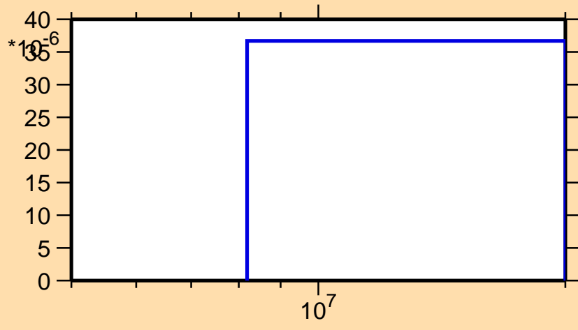
\sigma vs. E for ^{237}\text{Cm}(n,t)
