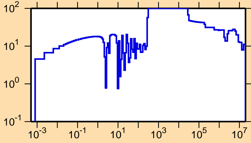
\Delta\sigma/\sigma vs. E for ^{238}\text{Cm}(n,tot.)
