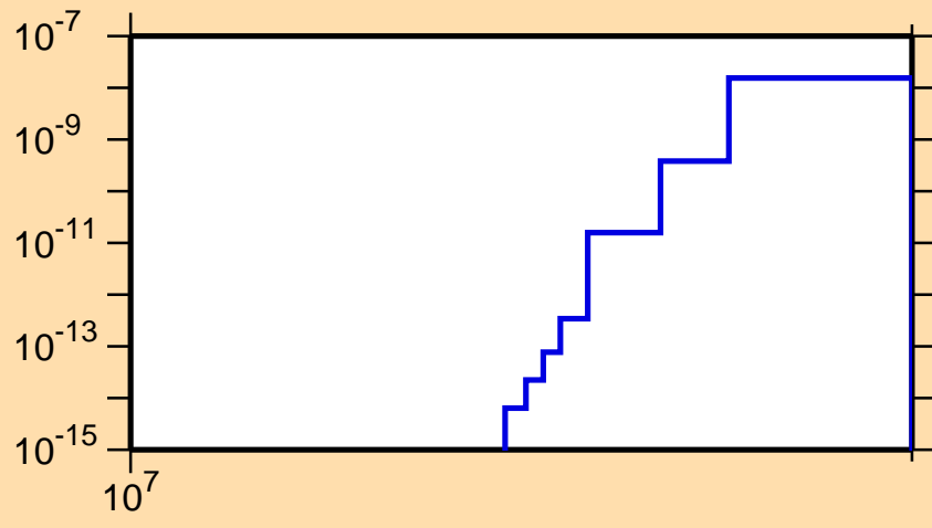
\sigma vs. E for ^{238}\text{Cm}(n,nd)
