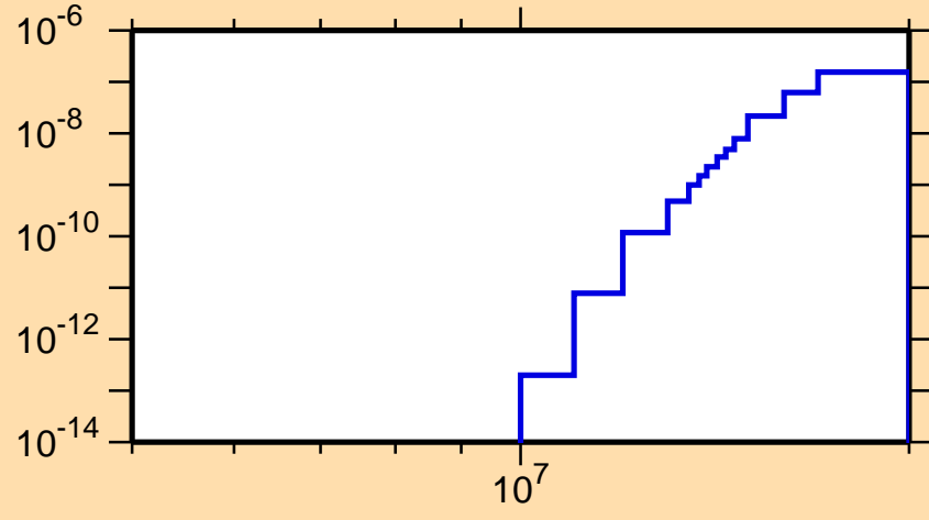
\sigma vs. E for ^{238}\text{Cm}(\text{mt117})
