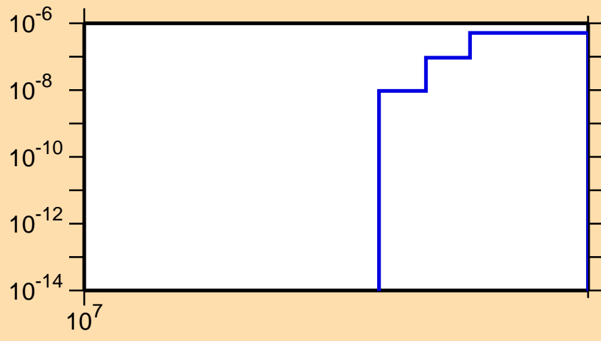
\sigma vs. E for ^{238}\text{Cm}(n,3n\alpha)
