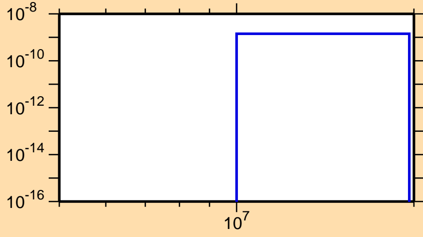
\sigma vs. E for ^{238}\text{Cm} (mt 45)
