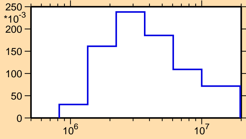
\sigma vs. E for ^{238}\text{Cm}(n,n\text{cont.})
