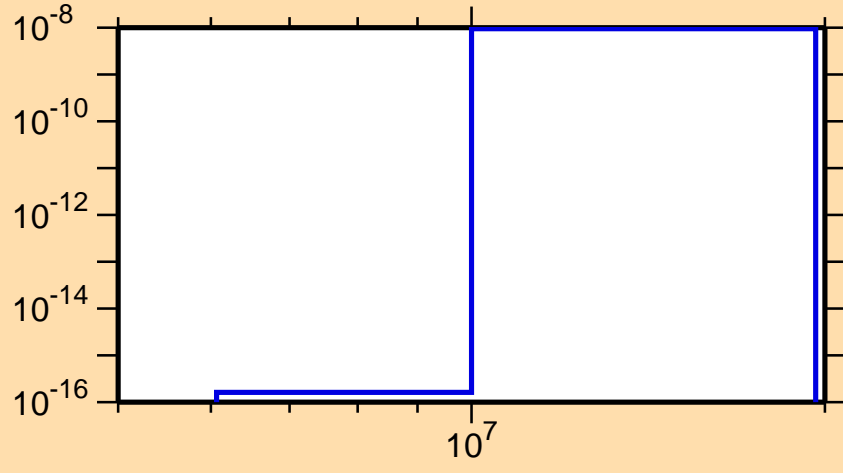
\sigma vs. E for ^{238}\text{Cm}(\text{mt117})
