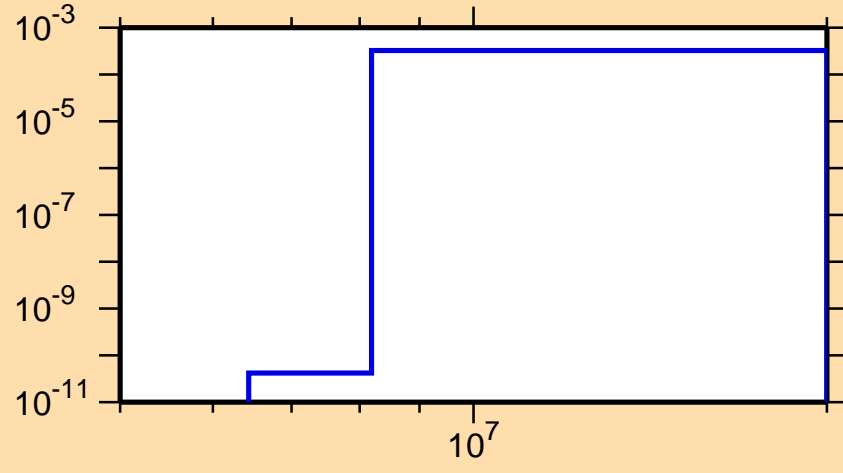
\sigma vs. E for ^{238}\text{Cm}(n,d)
