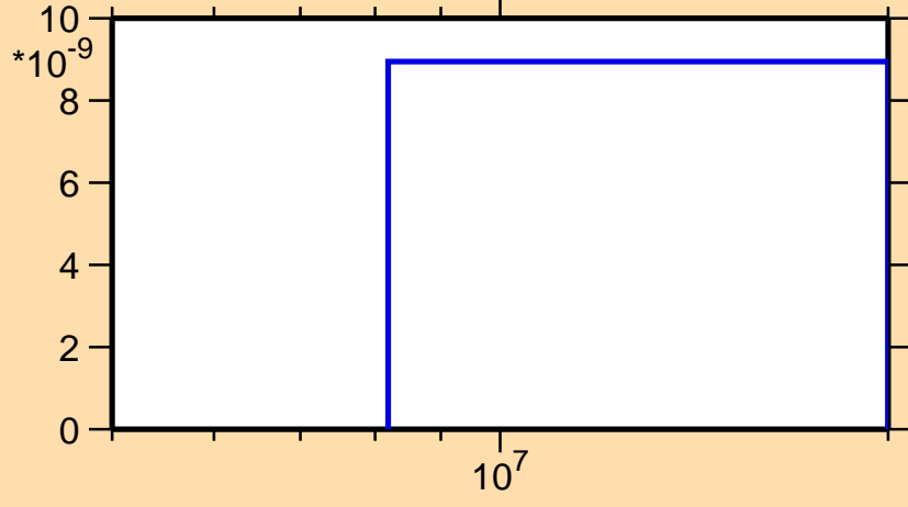
\sigma vs. E for ^{238}\text{Cm}(n,3n\alpha)
