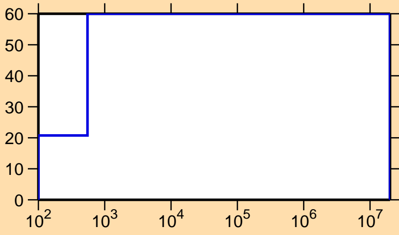
Delta \sigma/\sigma vs. E for ^{238}\text{Cm}(n,\gamma)
