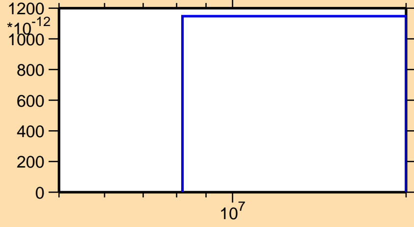
\sigma vs. E for ^{238}\text{Cm} (mt 45)
