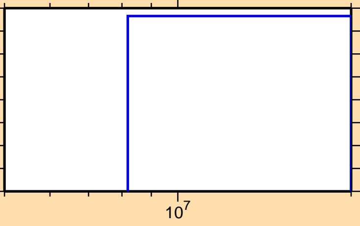
\sigma vs. E for ^{238}\text{Cm}(\text{mt117})
