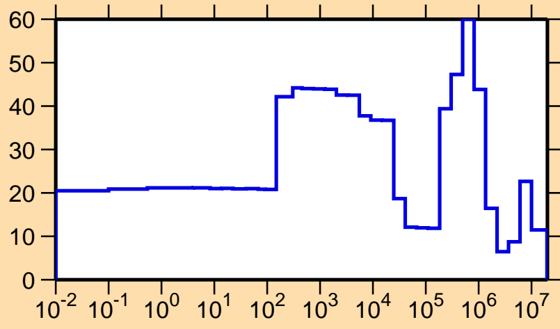
\Delta\sigma/\sigma vs. E for ^{239}\text{Cm}(n,el.)
