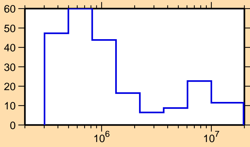
\Delta\sigma/\sigma vs. E for ^{239}\text{Cm}(n,\text{el.})
