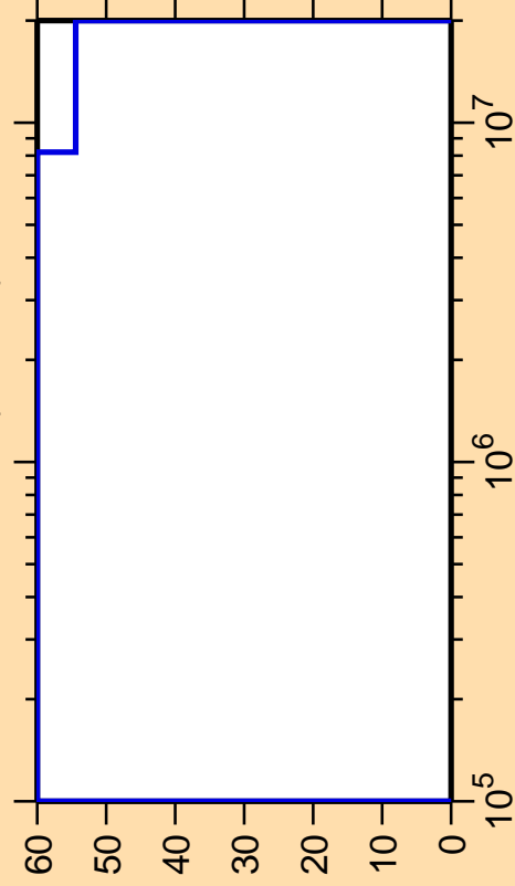
\Delta\sigma/\sigma vs. E for ^{239}\text{Cm}(n,\text{inel.})
