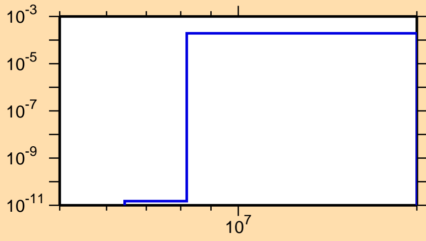
\sigma vs. E for ^{239}\text{Cm}(n,d)
