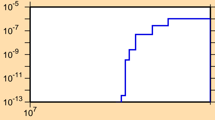
\sigma vs. E for ^{240}\text{Cm}(n,3n\alpha)
