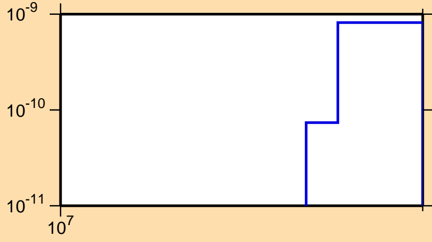
\sigma vs. E for ^{240}\text{Cm}(n,\text{He3})
