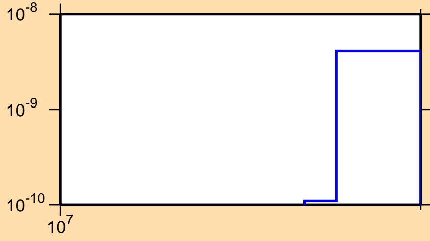
\sigma vs. E for ^{240}\text{Cm}(n,2np)
