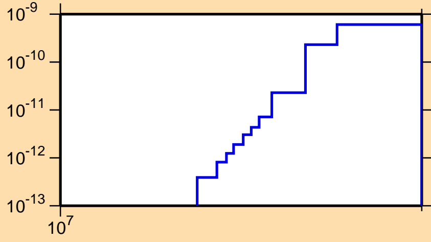
\sigma vs. E for ^{240}\text{Cm} (mt 45)
