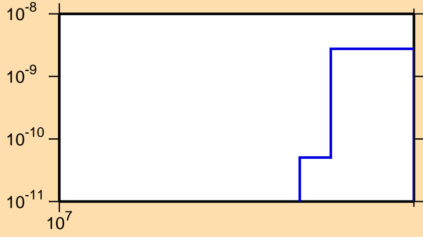
\sigma vs. E for ^{240}\text{Cm}(n,nt)
