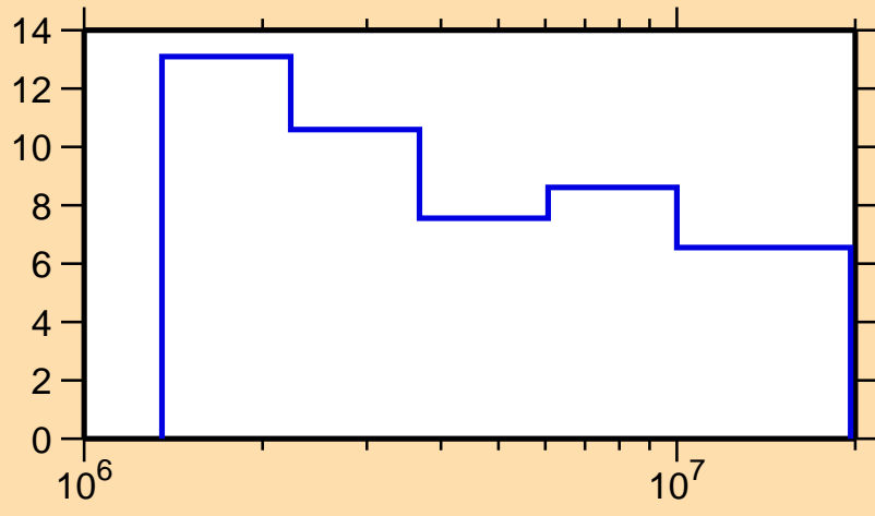
\Delta\sigma/\sigma vs. E for ^{240}\text{Cm}(n,f)
