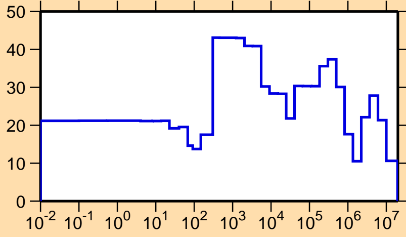
\Delta\sigma/\sigma vs. E for ^{240}\text{Cm}(n,el.)
