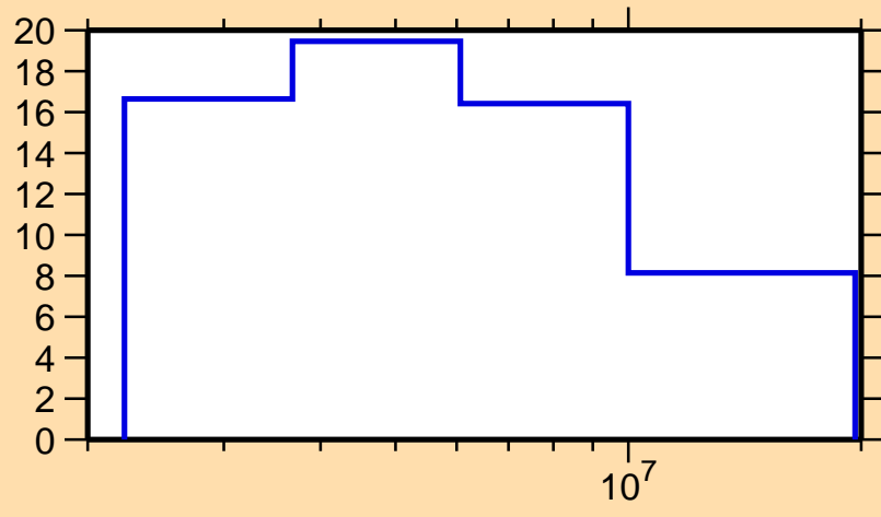
\Delta\sigma/\sigma vs. E for ^{240}\text{Cm}(n, tot.)
