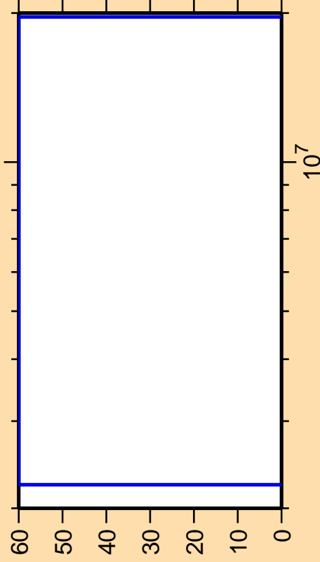
\Delta\sigma/\sigma vs. E for ^{240}\text{Cm}(n, ncont.)
