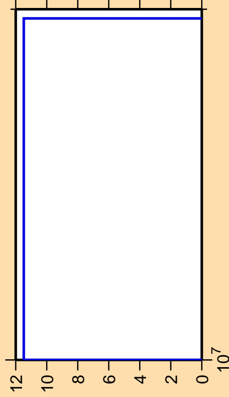
\Delta\sigma/\sigma vs. E for ^{240}\text{Cm} (mt 45)
