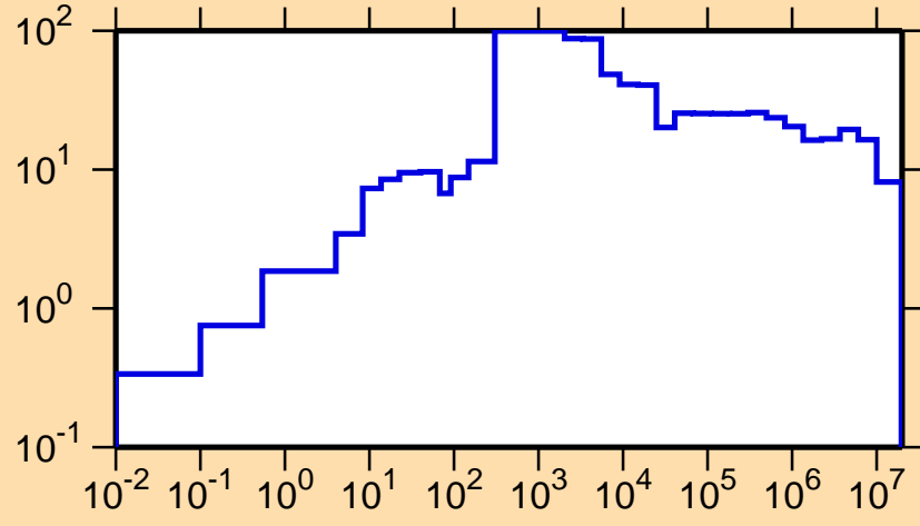
\Delta\sigma/\sigma vs. E for ^{240}\text{Cm}(n,tot.)
