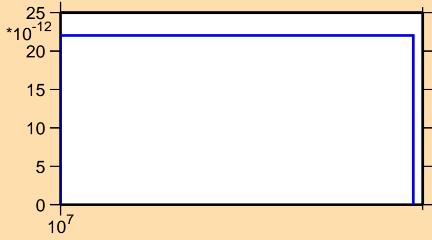
\sigma vs. E for ^{240}\text{Cm} (mt 45)
