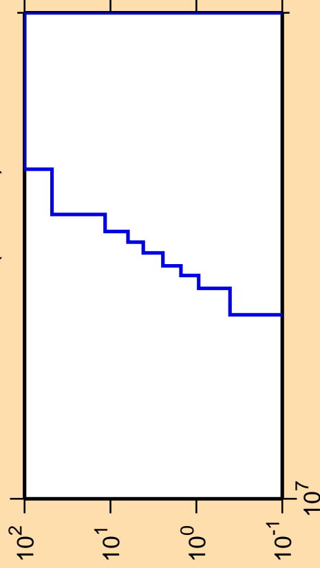
\Delta\sigma/\sigma vs. E for ^{241}\text{Cm}(\text{mt117})
