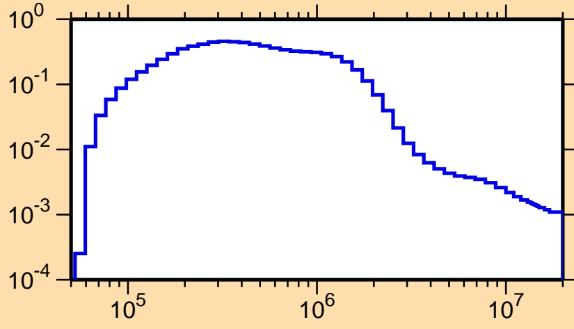
\sigma vs. E for ^{241}\text{Cm}(n,n_2)
