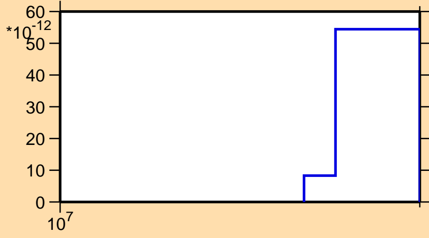
\sigma vs. E for ^{241}\text{Cm} (mt 45)
