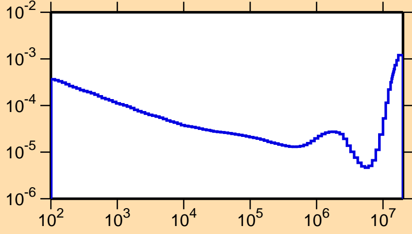
\sigma vs. E for ^{241}\text{Cm}(n,\alpha)
