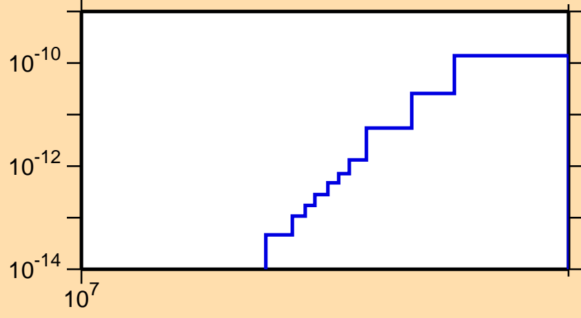
\sigma vs. E for ^{241}\text{Cm}(\text{mt117})
