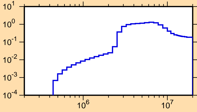
\sigma vs. E for ^{241}\text{Cm}(n,n\text{cont.})
