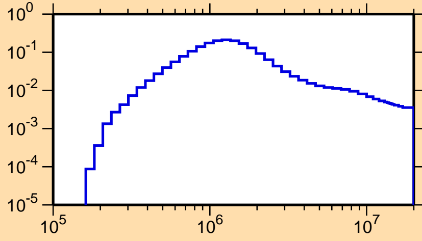
\sigma vs. E for ^{241}\text{Cm}(n,n_4)
