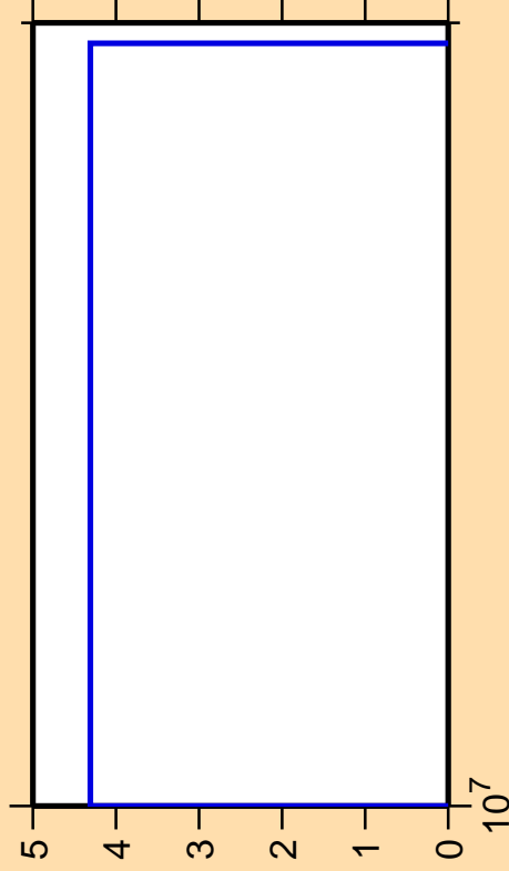
\Delta\sigma/\sigma vs. E for ^{241}\text{Cm}(n,\text{He3})
