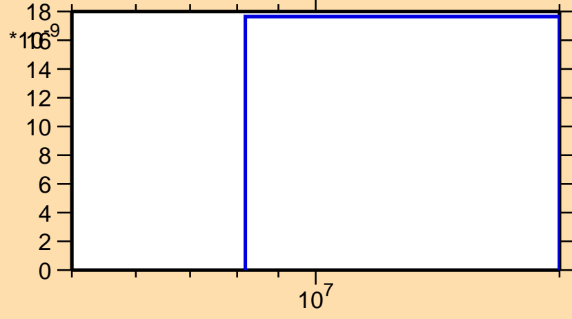
\sigma vs. E for ^{241}\text{Cm}(n,nd)
