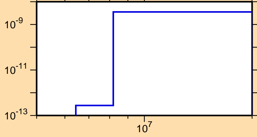
\sigma vs. E for ^{241}\text{Cm}(n,p\alpha)
