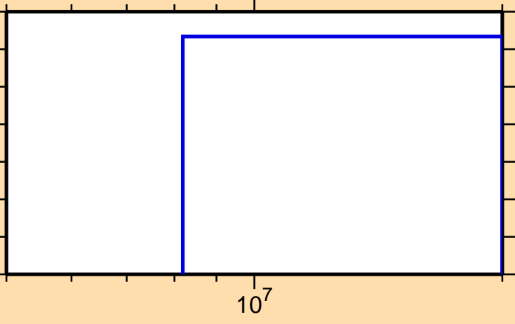
\sigma vs. E for ^{241}\text{Cm}(n,3n\alpha)
