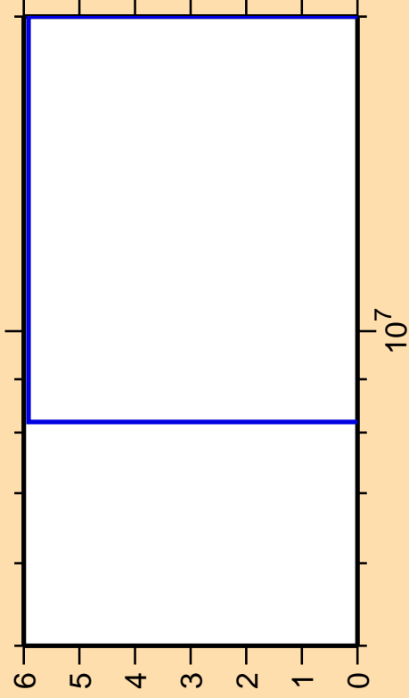
\Delta\sigma/\sigma vs. E for ^{241}\text{Cm} (mt 45)
