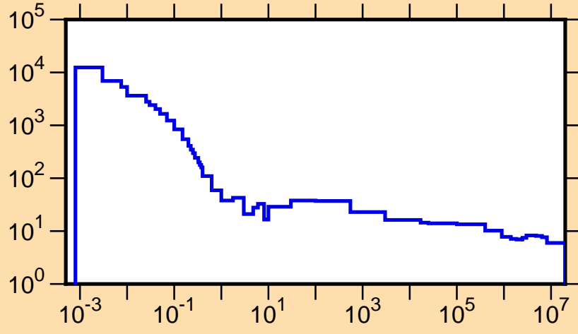
\sigma vs. E for ^{241}\text{Cm}(n,\text{tot.})
