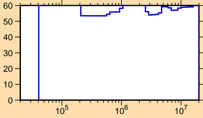
\Delta\sigma/\sigma vs. E for ^{242}\text{Cm}(n,n_1)
