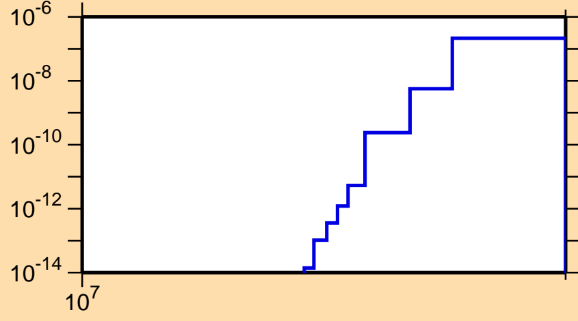
\sigma vs. E for ^{242}\text{Cm}(n,nd)
