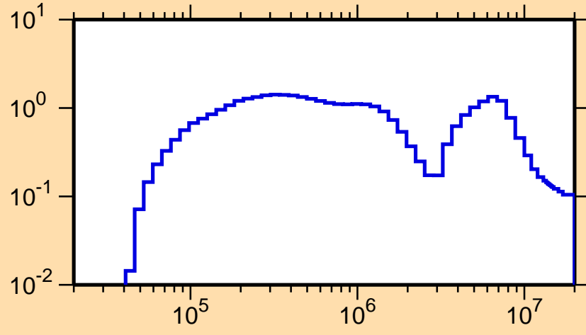
\sigma vs. E for ^{242}\text{Cm}(n,\text{inel.})
