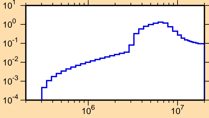
\sigma vs. E for ^{242}\text{Cm}(n,n\text{cont.})
