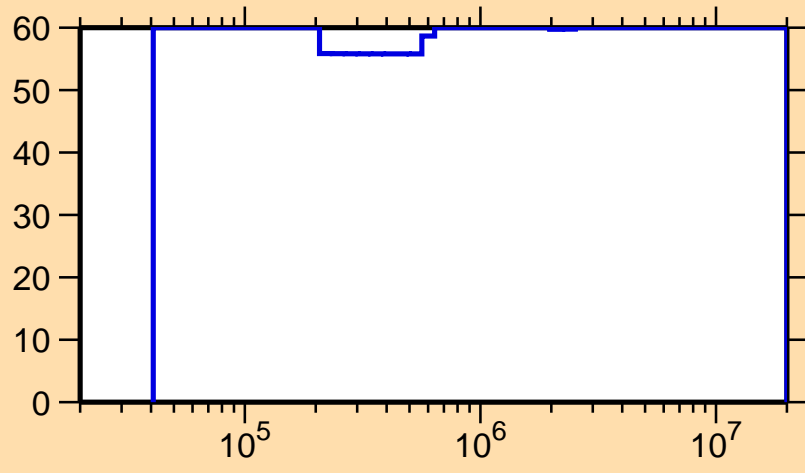
\Delta\sigma/\sigma vs. E for ^{242}\text{Cm}(n,\text{inel.})
