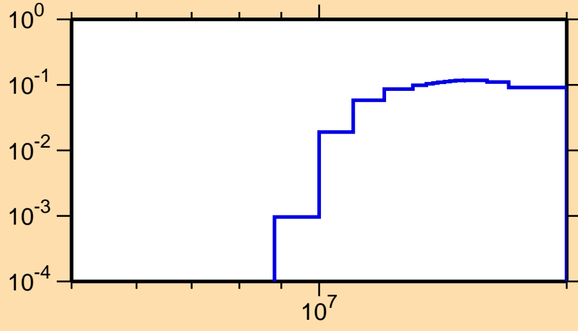
\sigma vs. E for ^{242}\text{Cm}(n,2n\alpha)
