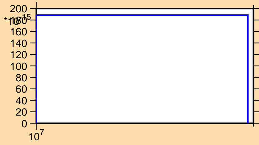
\sigma vs. E for ^{242}\text{Cm} (mt 45)
