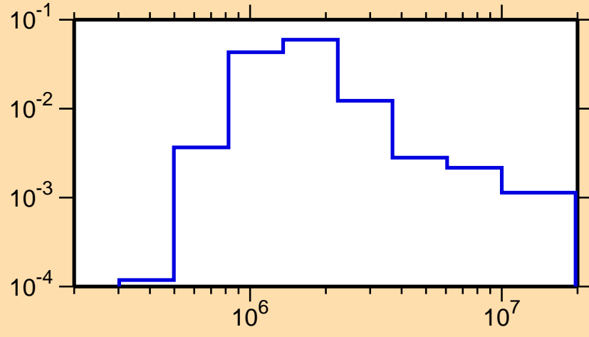
\sigma vs. E for ^{242}\text{Cm}(n,n_3)
