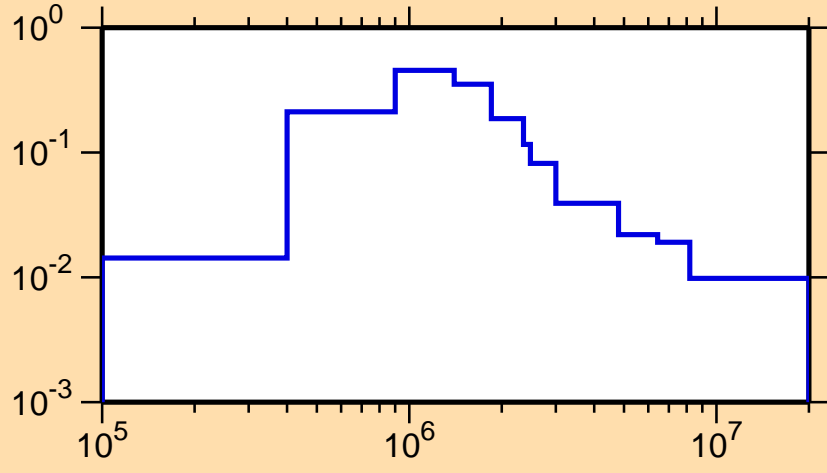
\sigma vs. E for ^{242}\text{Cm}(n,n_2)
