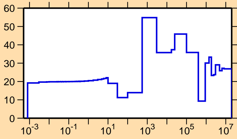
\Delta\sigma/\sigma vs. E for ^{242}\text{Cm}(n,el.)
