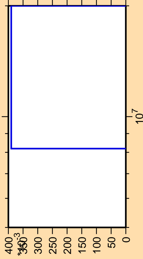
\Delta\sigma/\sigma vs. E for ^{242}\text{Cm} (mt 45)
