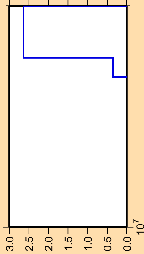
\Delta\sigma/\sigma vs. E for ^{243}\text{Cm} (mt 45)
