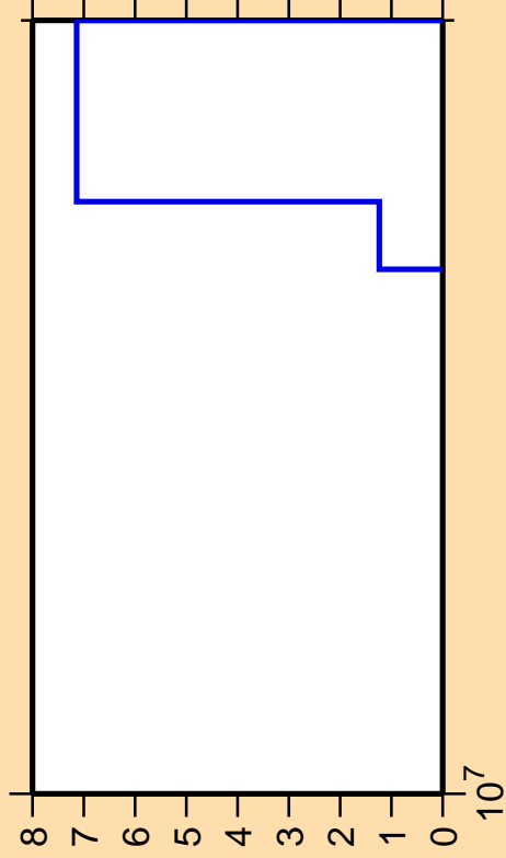
\Delta\sigma/\sigma vs. E for ^{243}\text{Cm}(\text{mt117})
