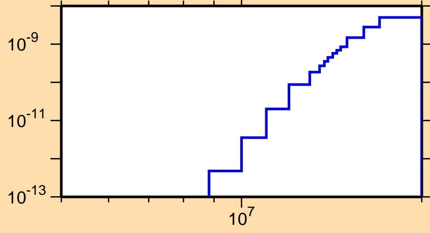
\sigma vs. E for ^{243}\text{Cm}(n,p\alpha)
