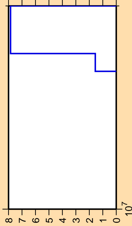
\Delta\sigma/\sigma vs. E for ^{243}\text{Cm}(n,\text{He}3)
