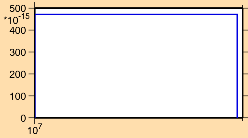
\sigma vs. E for ^{243}\text{Cm}(\text{mt117})
