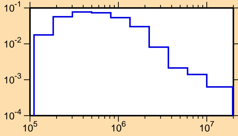
\sigma vs. E for ^{243}\text{Cm}(n,n_4)
