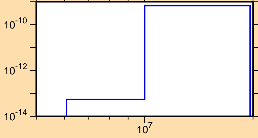
\sigma vs. E for ^{243}\text{Cm}(n,p\alpha)
