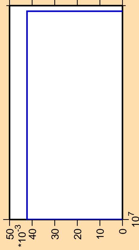
\Delta\sigma/\sigma vs. E for ^{243}\text{Cm} (mt 45)
