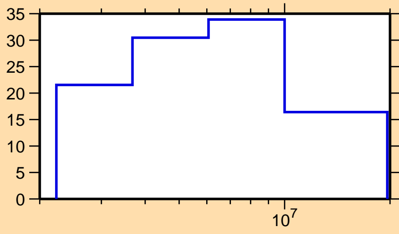
\Delta\sigma/\sigma vs. E for ^{243}\text{Cm}(n,ncont.)
