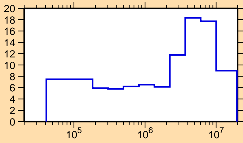
\Delta\sigma/\sigma vs. E for ^{243}\text{Cm}(n,inel.)
