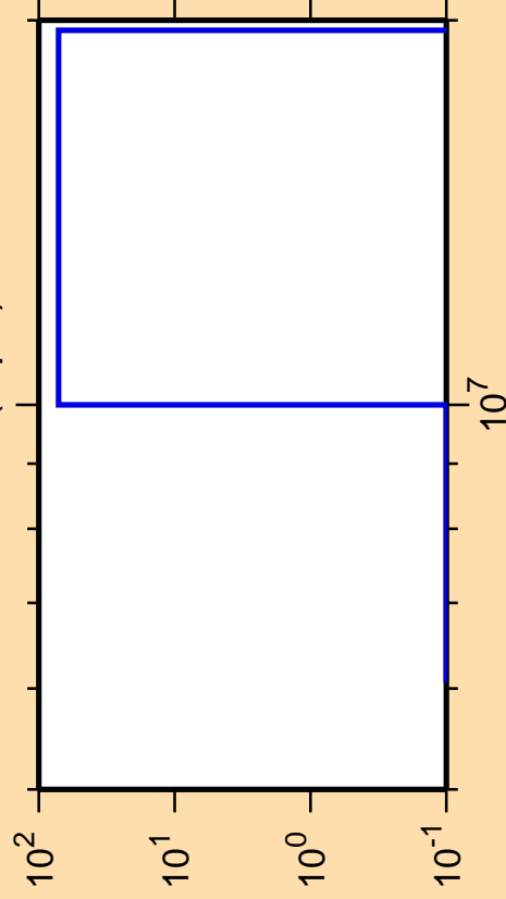
\Delta\sigma/\sigma vs. E for ^{243}\text{Cm}(n,p\alpha)
