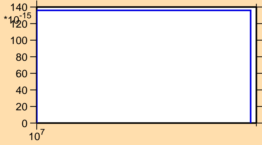
\sigma vs. E for ^{243}\text{Cm} (mt 45)
