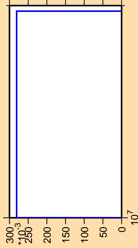
\Delta\sigma/\sigma vs. E for ^{243}\text{Cm}(n,\text{He}3)
