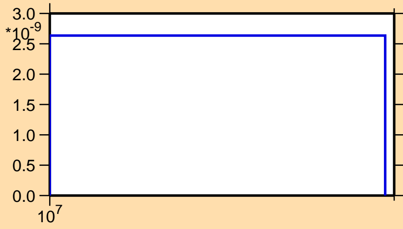
\sigma vs. E for ^{243}\text{Cm}(n,nt)
