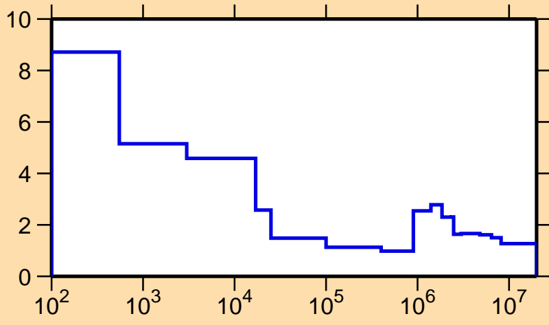
\Delta\sigma/\sigma vs. E for ^{243}\text{Cm}(n,\text{el.})
