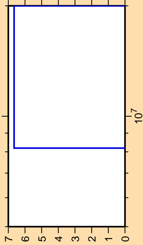
\Delta\sigma/\sigma vs. E for ^{243}\text{Cm}(n,np)
