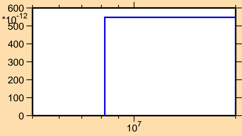
\sigma vs. E for ^{243}\text{Cm}(n,p\alpha)
