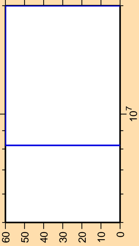
\Delta\sigma/\sigma vs. E for ^{243}\text{Cm}(n,p\alpha)
