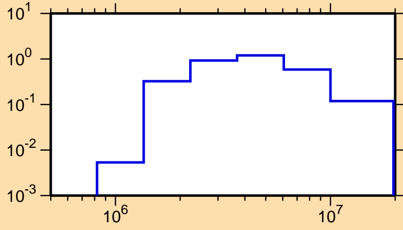
\sigma vs. E for ^{244}\text{Cm}(n,n\text{cont.})
