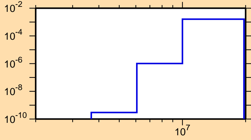
\sigma vs. E for ^{244}\text{Cm}(n,p)
