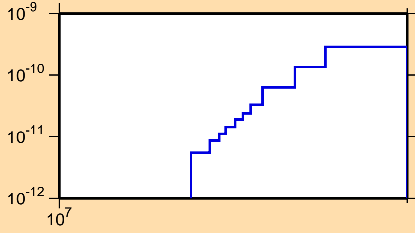
\sigma vs. E for ^{245}\text{Cm}(n,p\alpha)
