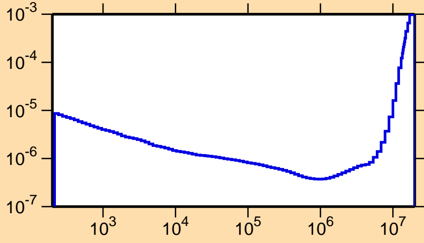
\sigma vs. E for ^{245}\text{Cm}(n,\alpha)
