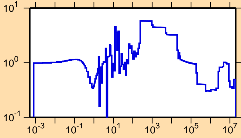
\Delta\sigma/\sigma vs. E for ^{245}\text{Cm}(n,tot.)
