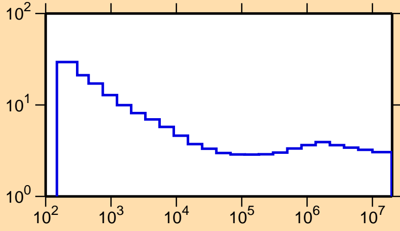
\sigma vs. E for ^{245}\text{Cm}(n,\text{nonel.})
