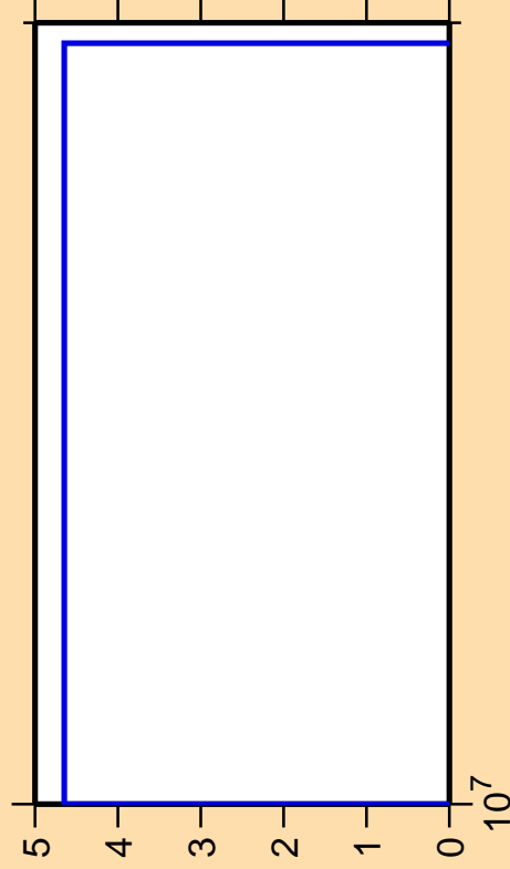
\Delta\sigma/\sigma vs. E for ^{245}\text{Cm}(n,p\alpha)
