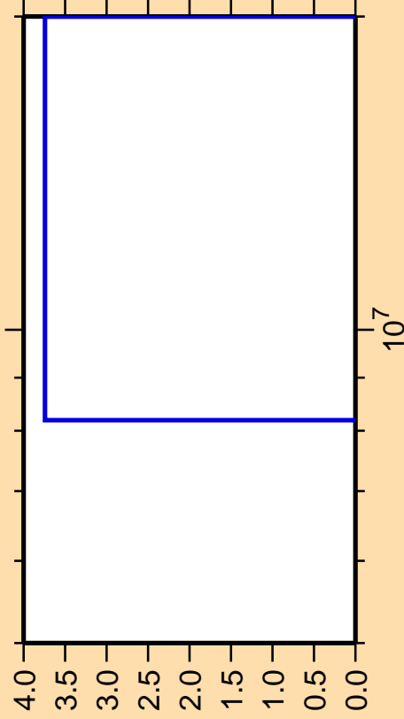
\Delta\sigma/\sigma vs. E for ^{245}\text{Cm}(n,p\alpha)
