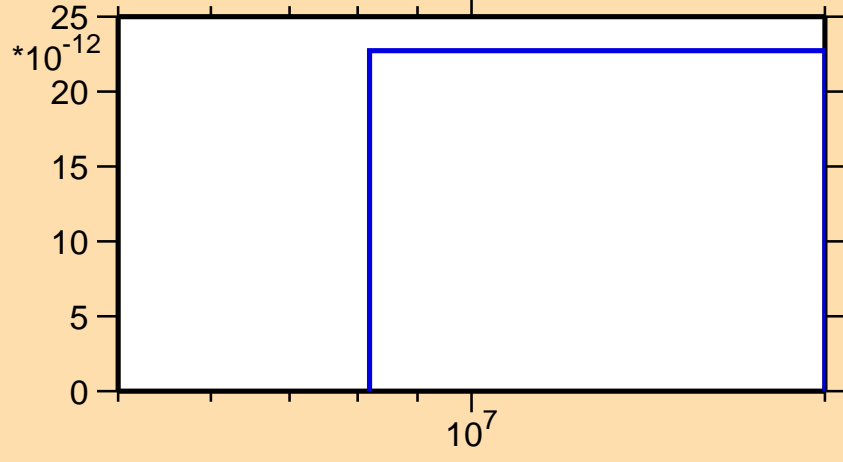
\sigma vs. E for ^{245}\text{Cm}(n,p\alpha)
