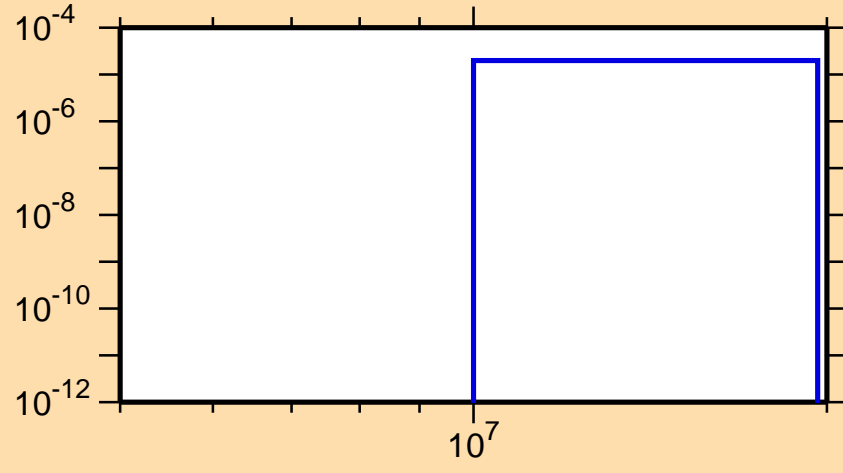
\sigma vs. E for ^{246}\text{Cm}(n,np)
