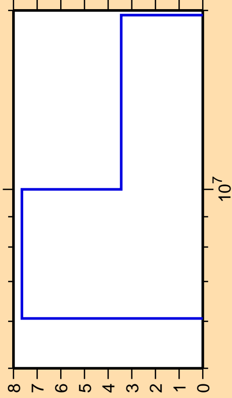
\Delta\sigma/\sigma vs. E for ^{246}\text{Cm}(n,\alpha)
