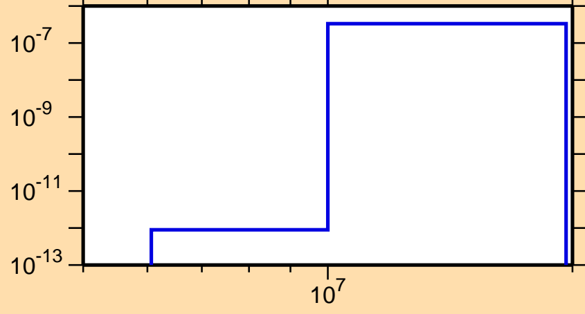
\sigma vs. E for ^{246}\text{Cm}(n,p\alpha)
