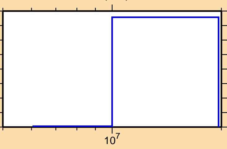
\sigma vs. E for ^{246}\text{Cm}(n,d)
