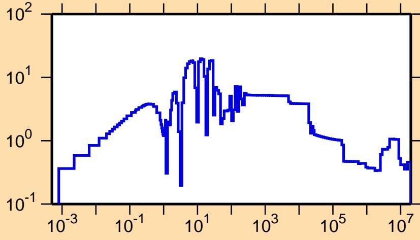
\Delta\sigma/\sigma vs. E for ^{247}\text{Cm}(n,tot.)
