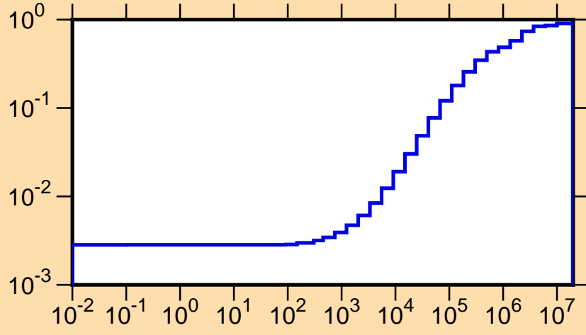
\mu vs. E for ^{247}\text{Cm}(\text{mt251})
