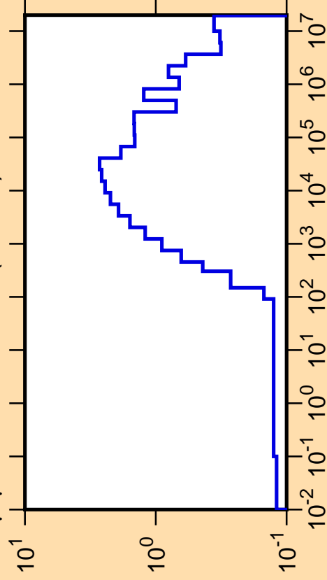
\Delta\mu/\mu vs. E for ^{247}\text{Cm}(\text{mt251})
