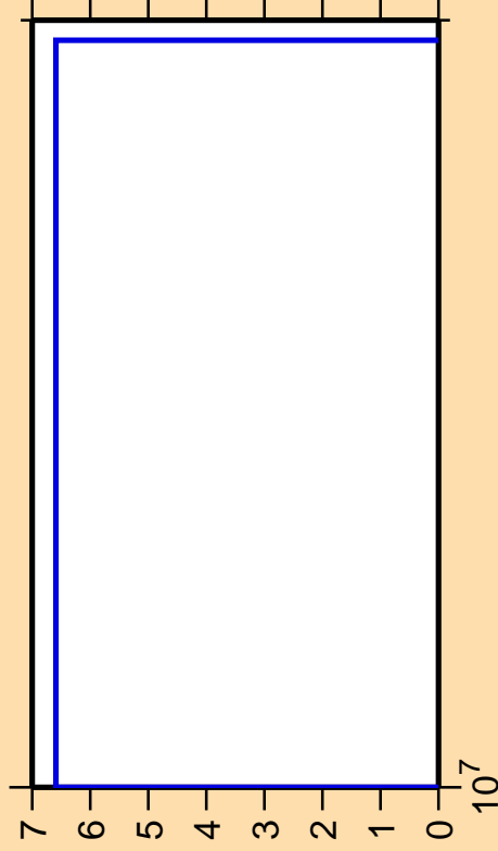
\Delta\sigma/\sigma vs. E for ^{247}\text{Cm}(n,3n\alpha)
