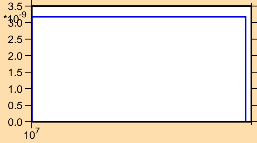
\sigma vs. E for ^{247}\text{Cm} (mt 45)
