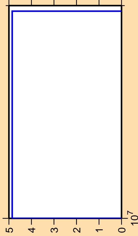
\Delta\sigma/\sigma vs. E for ^{247}\text{Cm}(n,nd)
