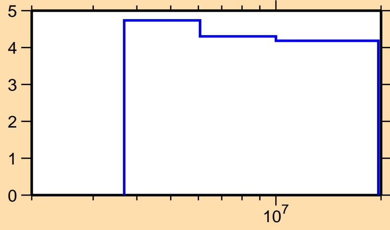
\Delta\sigma/\sigma vs. E for ^{247}\text{Cm}(n,p)
