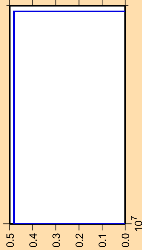
\Delta\sigma/\sigma vs. E for ^{247}\text{Cm}(n,p\alpha)
