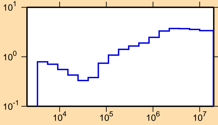
\sigma vs. E for ^{248}\text{Cm}(n,\text{nonel.})
