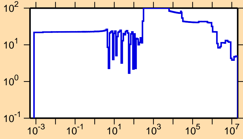
\Delta\sigma/\sigma vs. E for ^{249}\text{Cm}(n,el.)
