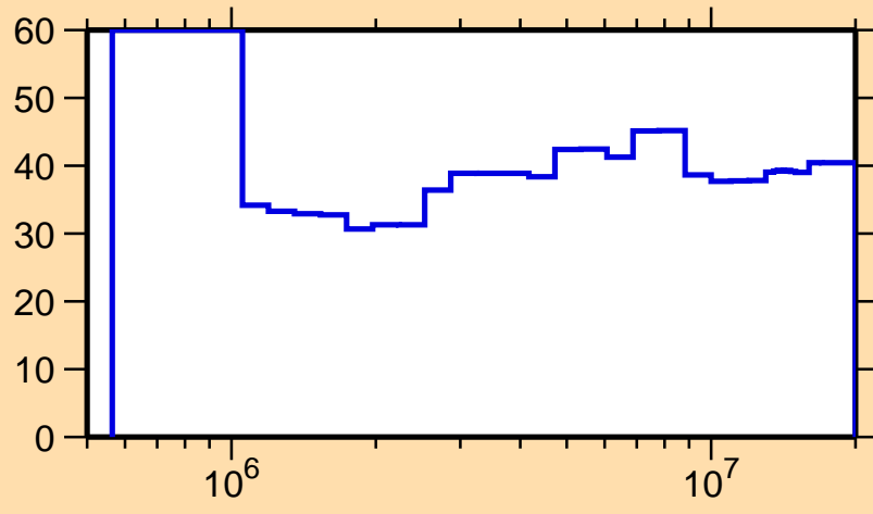
\Delta\sigma/\sigma vs. E for ^{249}\text{Cm}(n,ncont.)
