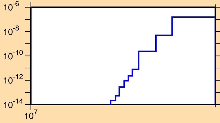
\sigma vs. E for ^{249}\text{Cm}(n,nt)
