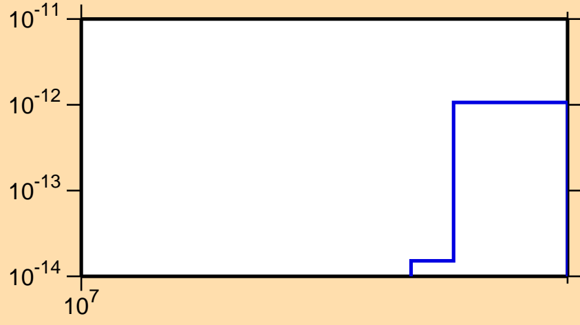
\sigma vs. E for ^{249}\text{Cm}(n,\text{He}3)
