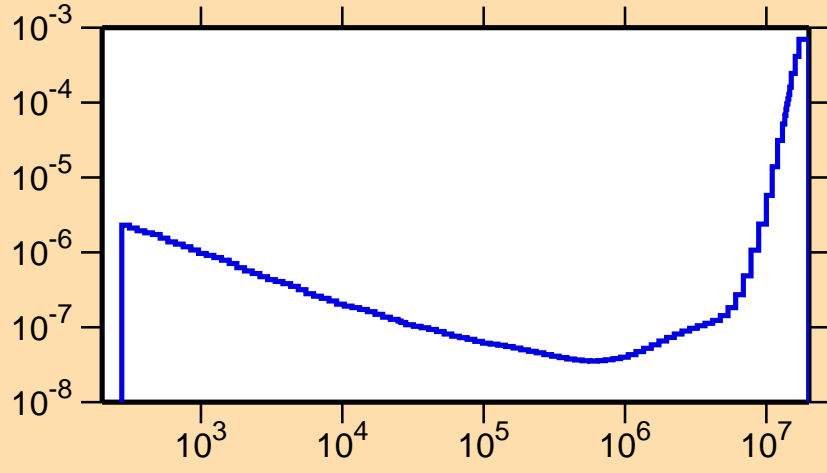
\sigma vs. E for ^{249}\text{Cm}(n,\alpha)
