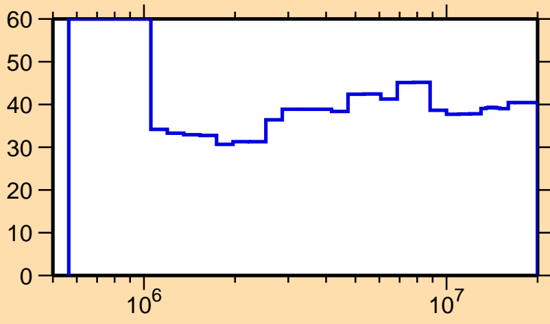
\Delta\sigma/\sigma vs. E for ^{249}\text{Cm}(n,n\text{cont.})
