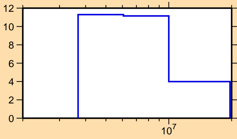
\Delta\sigma/\sigma vs. E for ^{249}\text{Cm}(n,\text{el.})
