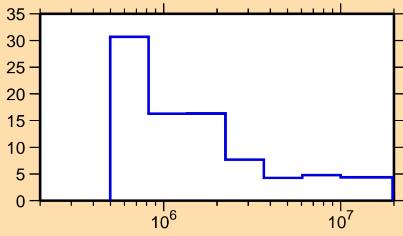
\Delta\sigma/\sigma vs. E for ^{249}\text{Cm}(n,\text{nonel.})
