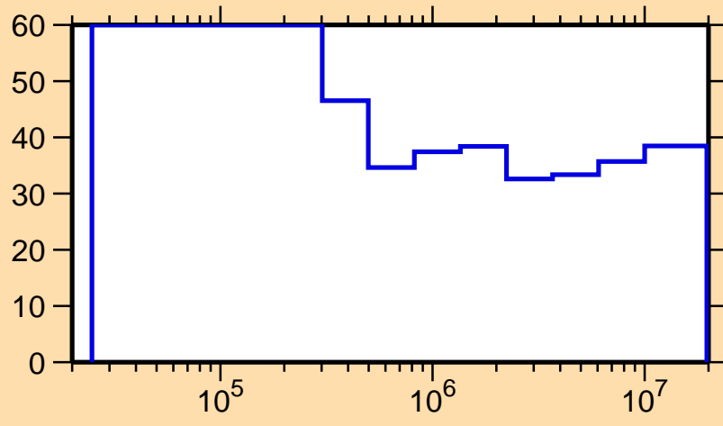
\Delta\sigma/\sigma vs. E for ^{249}\text{Cm}(n,n_1)
