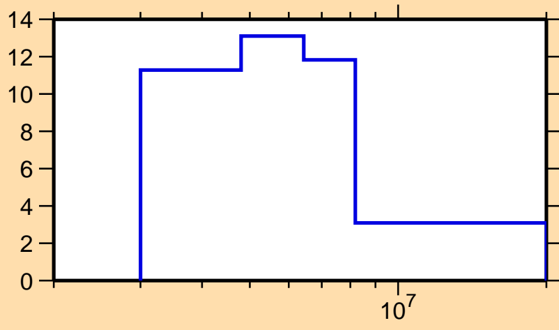
\Delta\sigma/\sigma vs. E for ^{249}\text{Cm}(n,el.)
